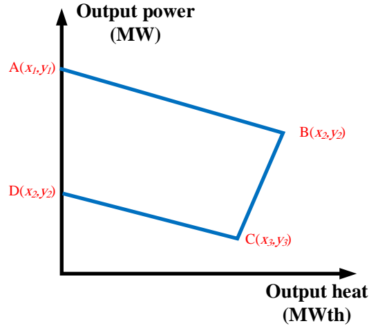
Fig. 2: Operation region of CHP unit.
