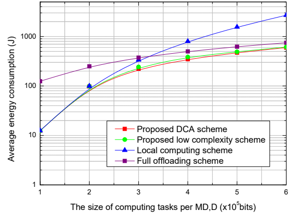
Fig. 4. The average energy consumption versus the size of computing tasks (20 MDs)
