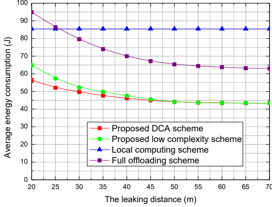
Fig. 5. The average energy consumption versus the leaking distance
