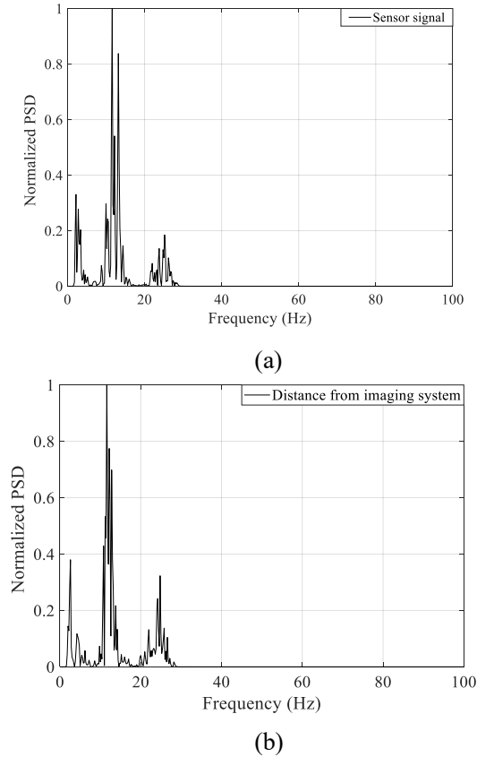
Fig. 10. Normalized PSD of the measurements in Fig. 9. (a) Signal from the electrostatic sensor. (b) Distance measured from the imaging system.
