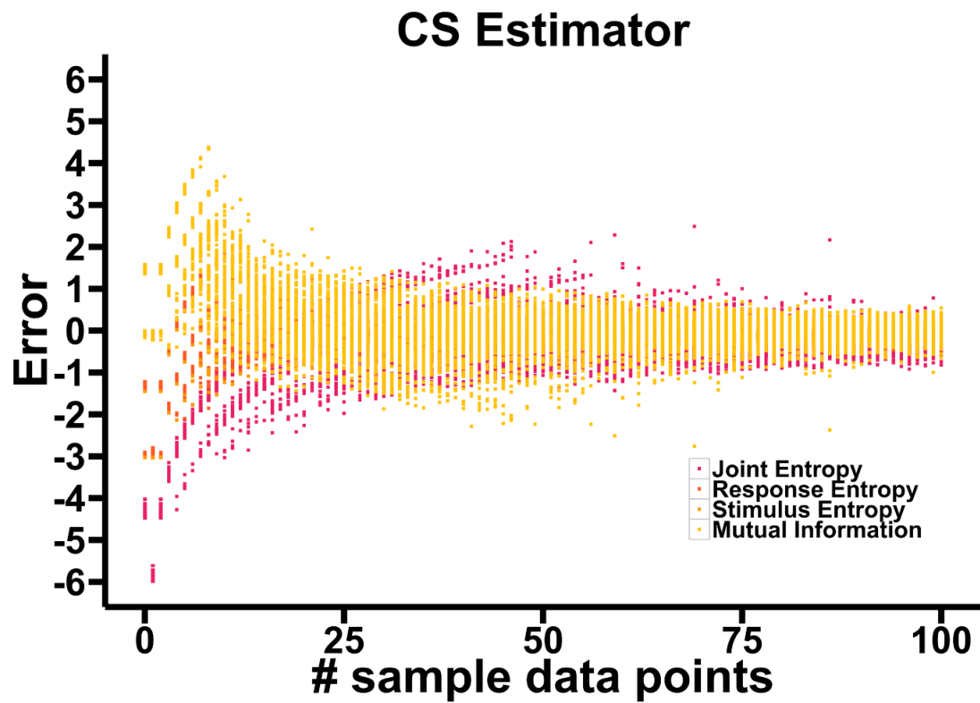
Figure 64) Error of the CS estimator from (Chao, Shen 2003) of stimulus, response and joint entropy, and mutual information for a range of different sample sizes from 1 to 100.
