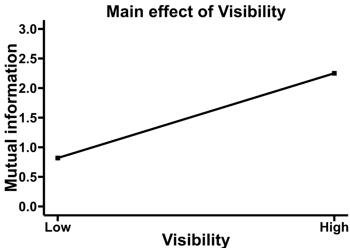
Figure 53) The effect of Visibility on Mutual Information. To illustrate this as clearly as possible, subject has been removed as a factor; MI is calculated based on a stimulus response matrix that is constructed across all Subjects.
