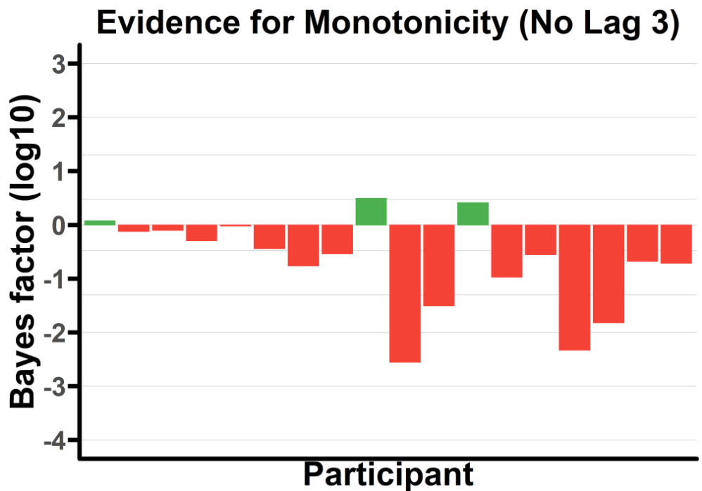
Figure 22) \log_{10} Bayes factors for monotonicity (positive, green) versus non-monotonicity (negative, red) across participants with lag 3 excluded. Note that participants are in the same order in all graphs to facilitate comparison. Lines overlaying the figure correspond to bayes factors of \frac{1}{100} , \frac{1}{20} , \frac{1}{3} , 3, 20 and 100 respectively.
