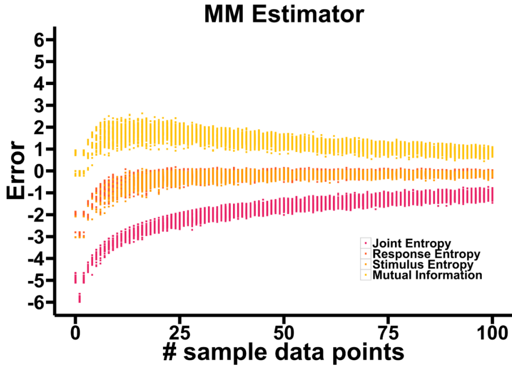
Figure 49) Error of the Miller-Madow estimator of stimulus, response and joint entropy, and mutual information for a range of different sample sizes from 1 to 100. Response and stimulus entropies are effectively identical, and so stimulus entropy (orange) overlays response entropy (red) on the plot.
