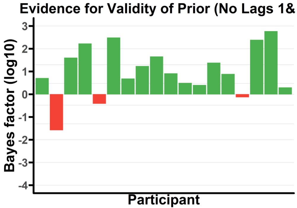
Figure 25) \log_{10} Bayes factors for positive evidence for the constraints (positive, green) versus negative evidence for constraints (negative, red) for empirical priors across participants with lags 1&2 excluded. Note that participants are in the same order in all graphs to facilitate comparison. Lines overlaying the figure correspond to bayes factors of \frac{1}{100} , \frac{1}{20} , \frac{1}{3} , 3, 20 and 100 respectively.
