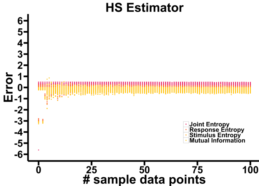
Figure 52) Error of the HS estimator of stimulus, response and joint entropy, and mutual information for a range of different sample sizes from 1 to 100. Response and stimulus entropies are effectively identical, and so stimulus entropy (orange) overlays response entropy (red) on the plot.
