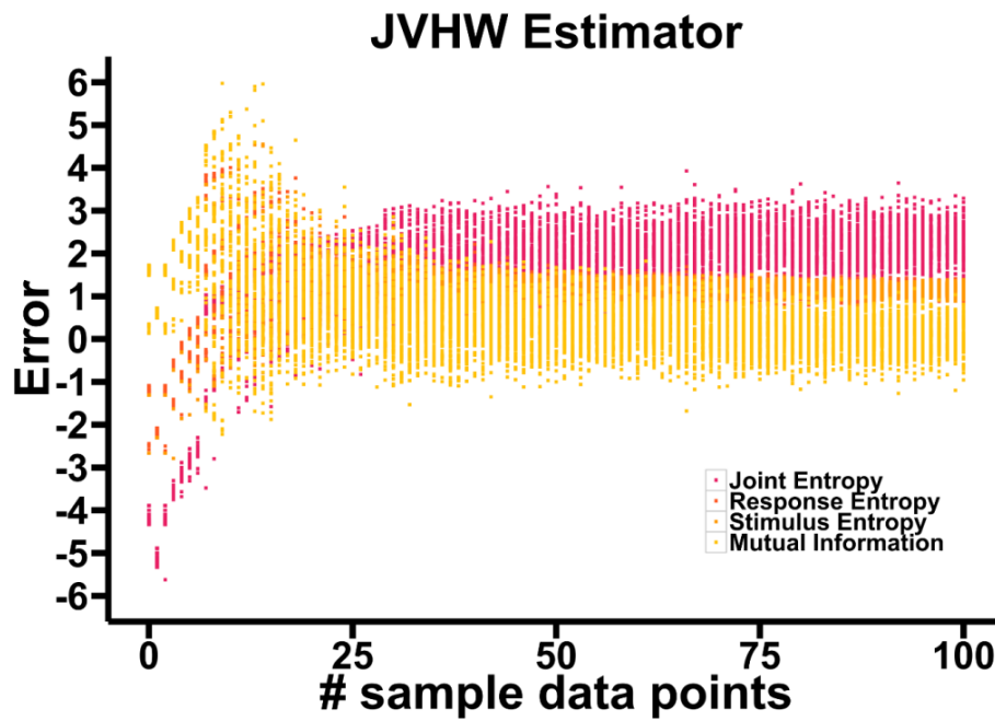
Figure 50) Error of the JVHW estimator of stimulus, response and joint entropy, and mutual information for a range of different sample sizes from 1 to 100. Response and stimulus entropies are effectively identical, and so stimulus entropy (orange) overlays response entropy (red) on the plot.
