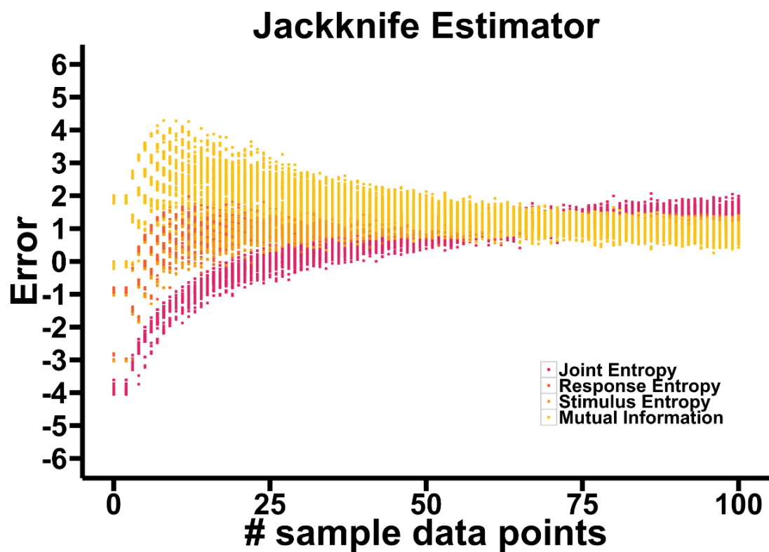
Figure 62) Error of the Jackknife entropy estimator described by (Paninski 2003) of stimulus, response and joint entropy, and mutual information for a range of different sample sizes from 1 to 100.
