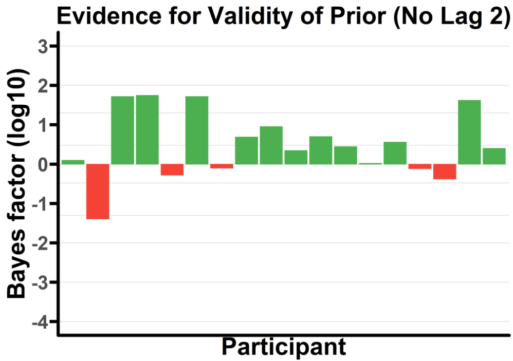
Figure 21) \log_{10} Bayes factors for positive evidence for the constraints (positive, green) versus negative evidence for constraints (negative, red) across participants with lag 2 excluded. Note that participants are in the same order in all graphs to facilitate comparison. Lines overlaying the figure correspond to bayes factors of \frac{1}{100} , \frac{1}{20} , \frac{1}{3} , 3, 20 and 100 respectively.
