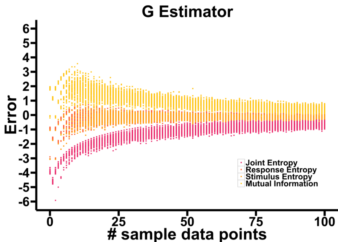
Figure 63) Error of the G estimator from (Grassberger 2003) of stimulus, response and joint entropy, and mutual information for a range of different sample sizes from 1 to 100.
