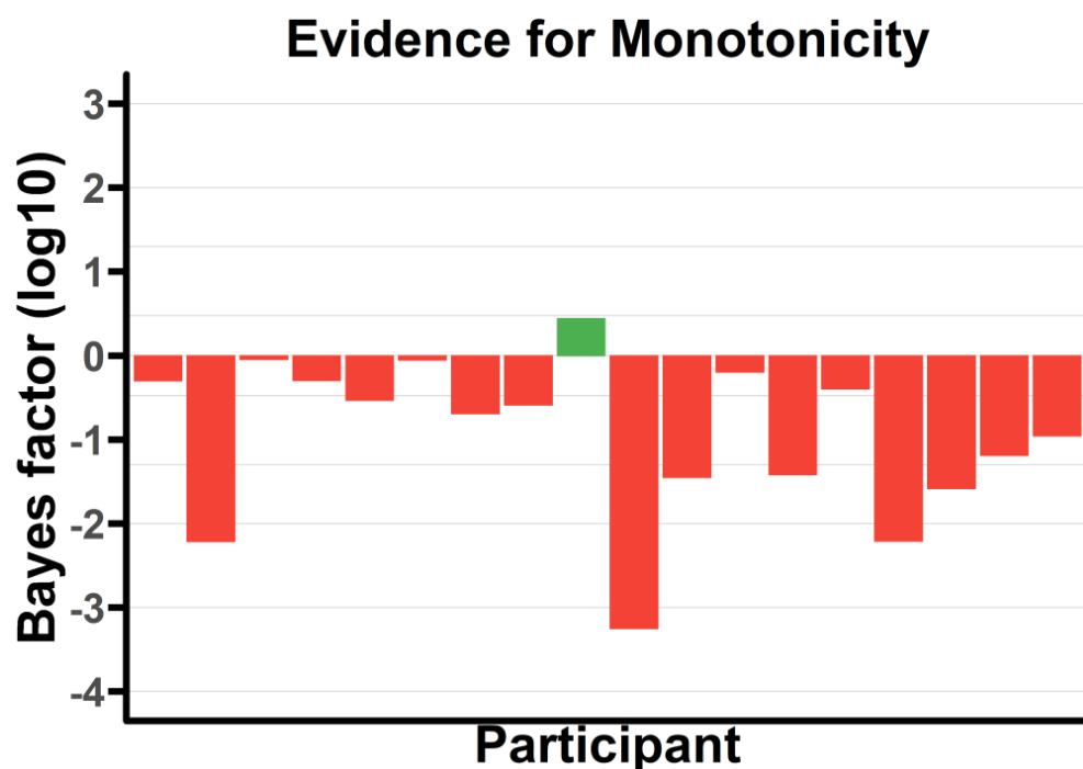
Figure 28) Log 10 Bayes factors for monotonicity (positive, green) versus non-monotonicity (negative, red) for empirical priors across participants. Note that participants are in the same order in all graphs to facilitate comparison. Lines overlaying the figure correspond to Bayes factors of \frac{1}{100} , \frac{1}{20} , \frac{1}{3} , 3, 20 and 100 respectively.
