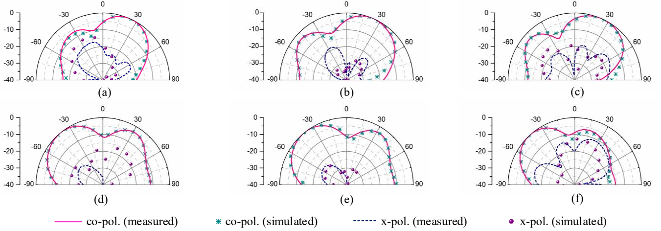
Fig. 18. Simulated and measured radiation patterns of the proposed multibeam array antenna with VP when port 1 is excited. (a)26.8 GHz @ quasi-E-plane. (b) 28 GHz @ quasi-E-plane. (c) 29.2 GHz @ quasi-E-plane. (d)26.8 GHz@ quasi-H-plane. (e)28 GHz @ quasi-H-plane. (f) 29.2 GHz @ quasi-H-plane.
