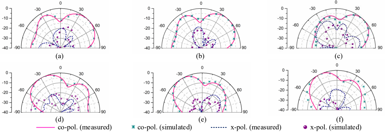
Fig. 19. Simulated and measured radiation patterns of the proposed multibeam array antenna with HP when port 5 is excited. (a)26.8 GHz @ quasi-E-plane. (b) 28 GHz@ quasi-E-plane. (c) 29.2 GHz @ quasi-E-plane. (d)26.8 GHz @ quasi-H-plane. (e)28 GHz @ quasi-H-plane. (f) 29.2 GHz @ quasi-H-plane.
