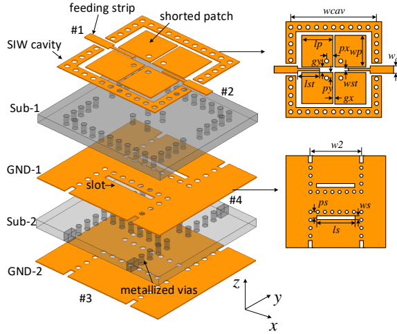
Fig. 1. Configuration of the proposed differentially-fed dual-polarized antenna. (Dimensions: w_{cav} = 6.4 mm, l_p = 2.2 mm, w_p = 2.2 mm, g_x = 0.15 mm, g_y = 0.4 mm, p_x = 0.425 mm, p_y = 0.4 mm, l_{st} = 1.55 mm, w_{st} = 0.15 mm, and w_1 = 0.5 mm, w_2 = 4.3 mm, l_s = 3.2 mm, w_s = 0.3 mm, and p_s = 0.5 mm)
