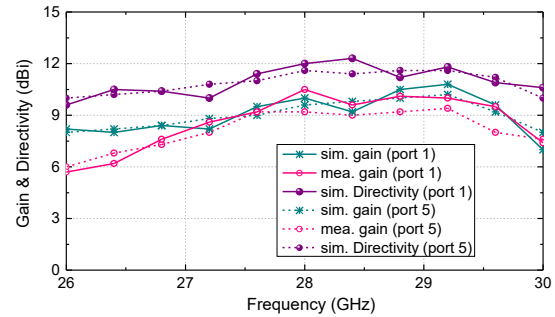
Fig. 21. Simulated gain, directivity and measured gain when port #1 and port #5 is excited, respectively.
