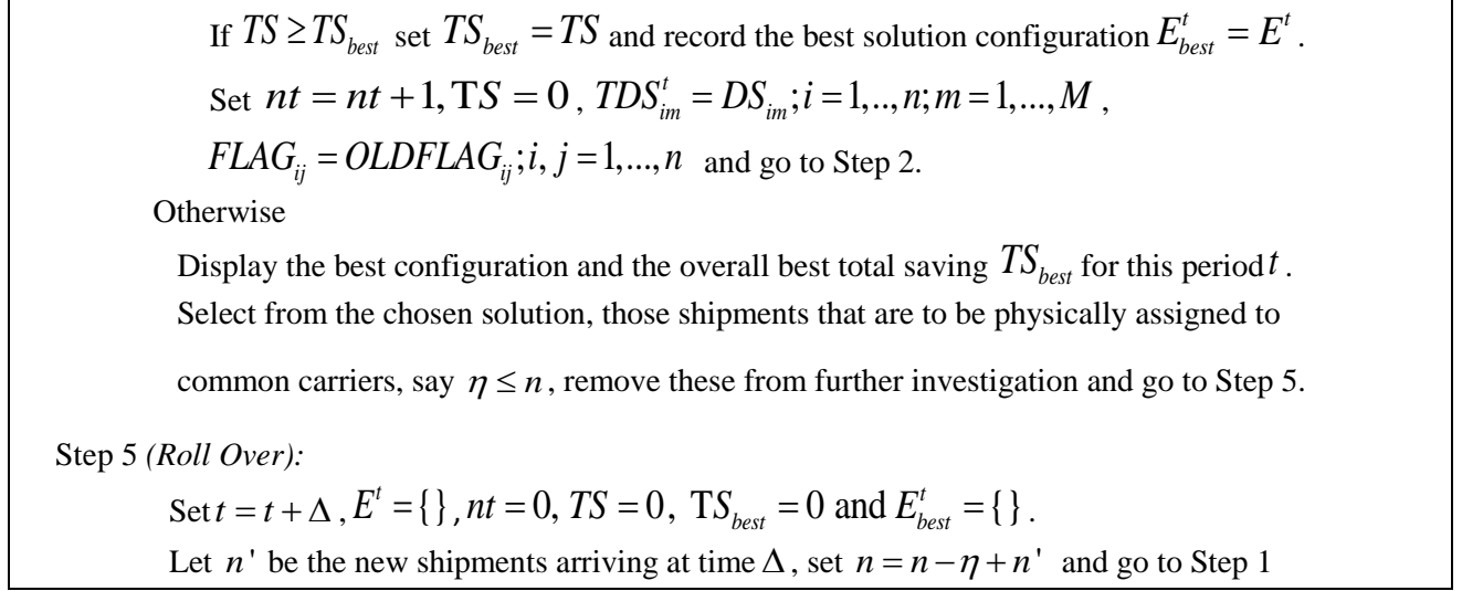
Figure 8: A Real Time GRASP-Based Meta-Heuristic
