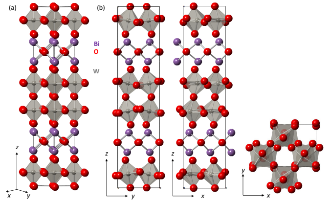
FIG. 1. The structure of Bi 2 W 2 O 9 in (a) the aristotype paraelectric I4/mmm phase and (b) the distorted orthorhombic Pnab ground state showing rotation of WO_6 octahedra about in-plane and out-of-plane axes and in-plane antipolar displacements of W^{6+} ions. Bi, W and O ions are shown in purple, grey and red, respectively, and corner-linked WO_6 octahedra in grey.
