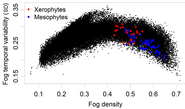
Figure 6. A scatterplot of fog density and fog temporal variability. The curvilinear relationship shows increasing and high temporal fog variability in areas with low fog densities (<0.4) but lower and decreasing fog variability in areas of high fog densities. Fog density is significantly higher ( P < 0.001 ) and temporal variability lower for mesophytes compared to xerophytes, providing evidence that the fog density layer is accurate.
