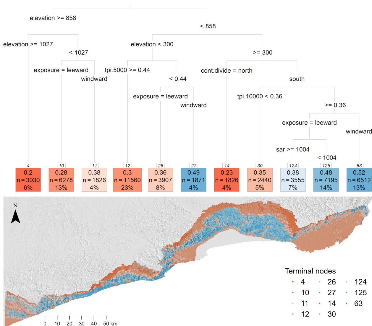
Figure 8. Tree describing fog distributions had 10 splits, 11 terminal nodes and a cross-validated error of 0.582. The ‘jumps’ in the node numbers result from the pruning of those branches which did not decrease the overall lack of fit by a factor of complexity parameter. The terminal node numbers were reassigned to the data points and mapped according to the tree colour scheme.
