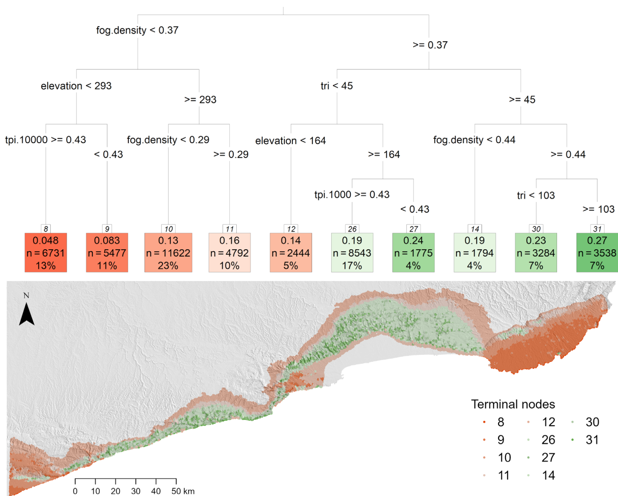
Figure 9. The tree describing vegetation distributions had 9 splits, 10 terminal nodes and a cross-validated error of 0.349. The 'jumps' in the node numbers result from the pruning of those branches which did not decrease the overall lack of fit by a factor of complexity parameter. The terminal node numbers were reassigned to the data points and mapped according to the tree colour scheme.
