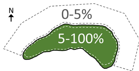
Figure 2. A diagram illustrating the criteria employed for filtering out scenes with little or no fog (<5% over the mountains) or a high coverage of mid-level or high-level clouds (>5% to the north of the mountains) prior to calculating the average fog density. One hundred and nineteen of 251 Landsat 5 scenes, 17 of 36 Landsat 7 scenes and 121 of 232 Landsat 8 scenes remained after removing fogless and cloudy scenes.
