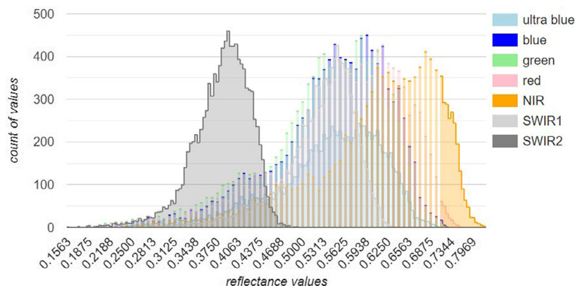
Figure 3. Histograms of the band reflectance values in fog areas. The NIR band detects the greatest range of reflectance values in fog areas, and thus the range of fog densities are well-represented.
