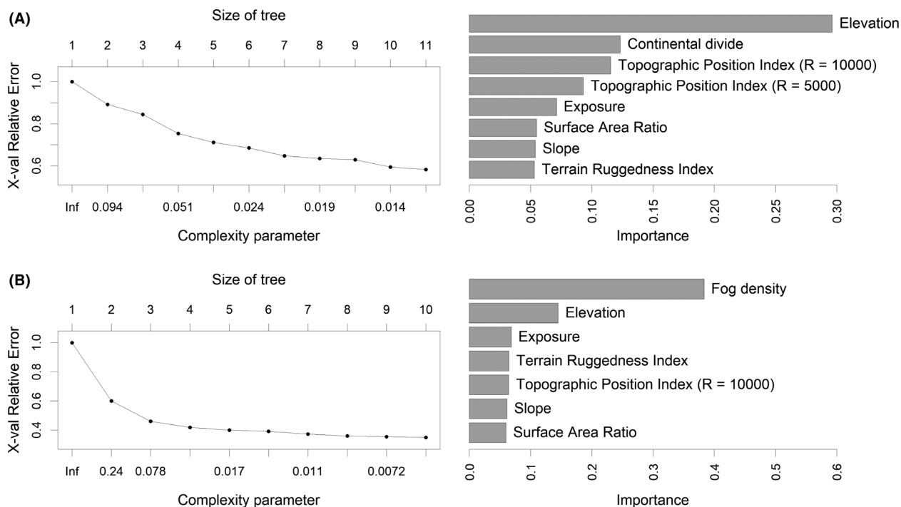
Figure 10. Complexity parameter plots and variable importance for (A) the tree describing fog distributions and (B) the tree describing vegetation distributions. Complexity parameter plots show the reduction in the cross validated error with decreasing complexity parameter and increasing tree size. We would see diminishing returns if we continued to grow the trees. Variable importance is calculated as the sum of the goodness of split measures (Gini index) and considers both primary and surrogate splits.
