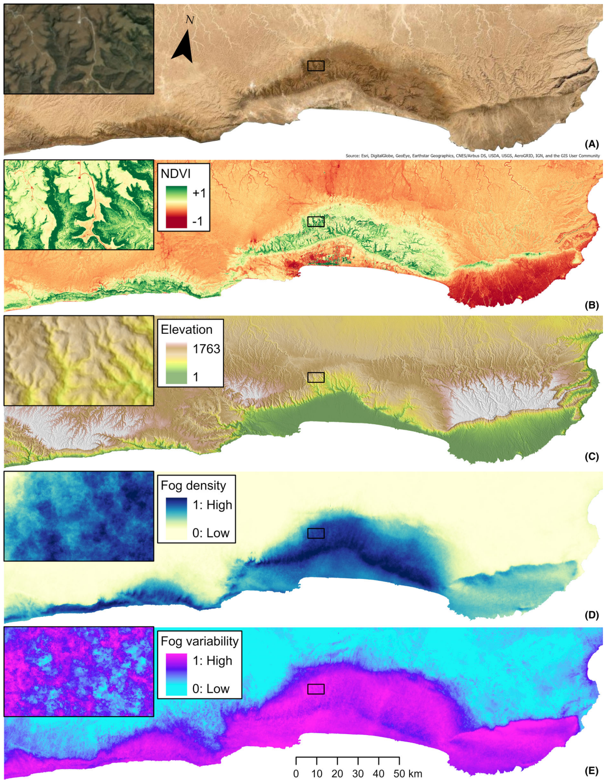
Figure 5. Layers of (A) true-colour satellite image, (B) NDVI, (C) elevation, (D) average fog density and (E) fog temporal variability, for the central South Arabian mountains. Broad-scale correlative patterns are evident. Difference in NDVI between cloud forest and grassland can be seen in the inset maps.
