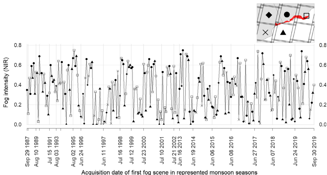
Figure 4. Number of scenes (total 257) and their locations (WRS-2 path/row) in each represented monsoon season (1987–2002 and 2013–2019). Fog intensity was calculated for each scene as the mean of the fog density cell values within an analysis window. Each tile area (WRS-2 path/row) contained an analysis window, within which every scene had complete data.
