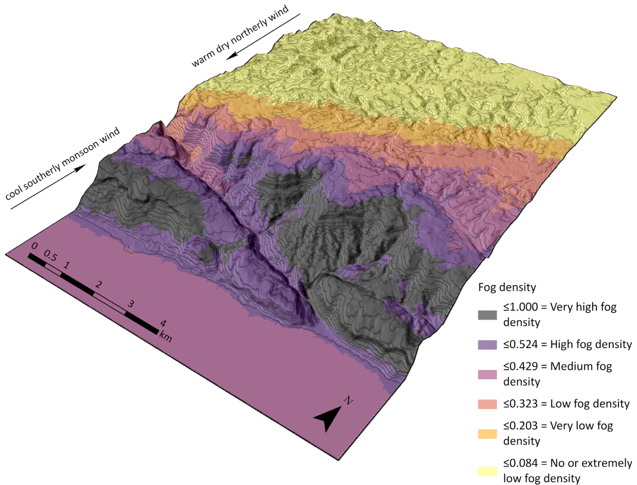
Figure 7. A three-dimensional cross section of the central South Arabian mountains between Dhalkut and Rakhyut in Dhofar, with the layer of fog density draped over a double-exaggerated, contoured, shaded relief elevation surface. Fog density has been classified into six classes (Jenks optimization). Steep windward slopes obstruct the inland movement of fog affecting its distribution.
