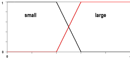
Fig. 4. Membership functions of input Sepal Length with two MFs.
