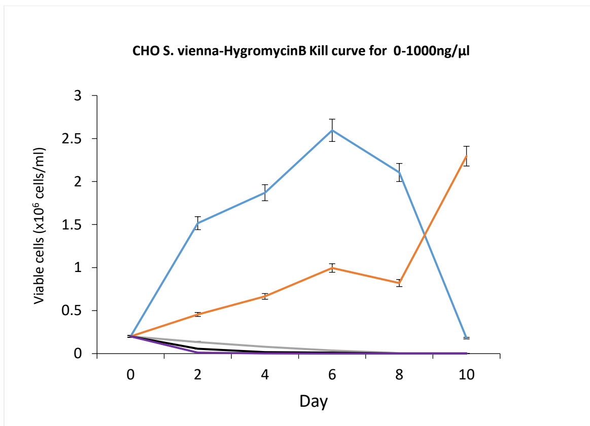
Figure 2.1 Hygromycin B Kill Curve for stable cell line generation. Selected transfected cells were selected using optimal antibiotic concentration, which is the lowest concentration that kills cells with 14 days. Here, 750 ng/ \mu l was the optimal concentration used for this study. Error bars represent percentage among biological triplicates (where n = 3).
