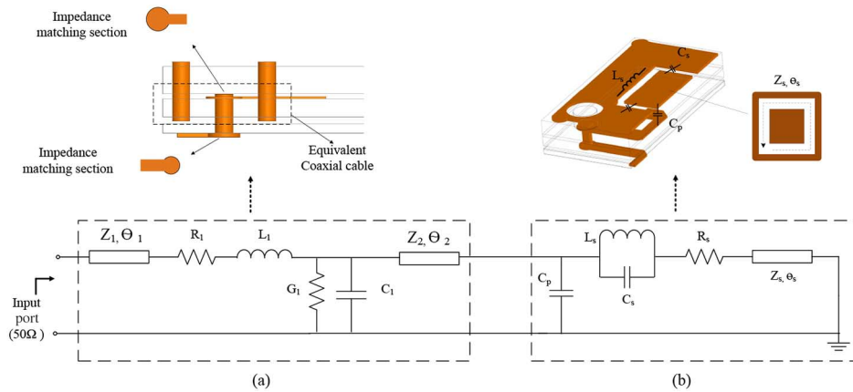
Fig. 10. Equivalent circuit model of the (a) stripline to microstrip transition and (b) ring-slot antenna.
