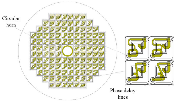
Fig. 18. Back view of the passive folded reflectarray.
