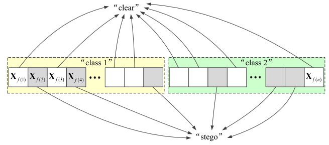
FIGURE 4. Labels of images for detection.
