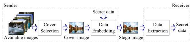
FIGURE 1. Cover selection based steganography.
