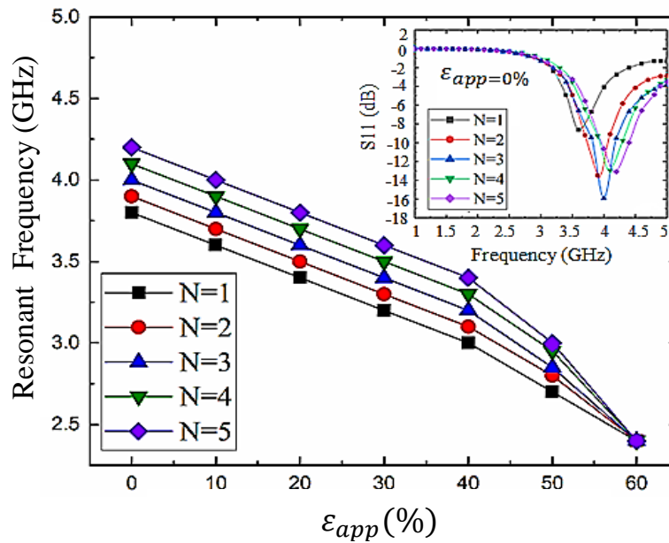
Fig. 6. Resonant frequency shift vs strain value in the PDMS substrate for the half wave length dipole antenna with buckled sections N = 1 to N=5 . Inset figure presents reflection coefficient (dB) versus frequency (GHz) for the sensor in the relaxed mode with unswollen PDMS and shows a good antenna match with N=2 and N=3 .
