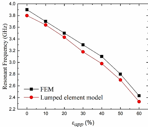
Fig. 4. Resonant frequency as a function of strain value in PDMS ( \epsilon_{app} ). Plot compares the results from numerical simulation in COMSOL and predictions from geometry-based model. Note that N=2 in this study.
