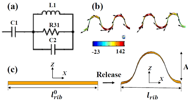
Fig. 3 (a) Equivalent circuit model used for modeling popup dipole antenna [38], (b) Surface current (A/m) on the buckling dipole after deswelling and returning to the original PDMS size, (c) Diagram of mechanics model for a meander section of a buckled ribbon.
