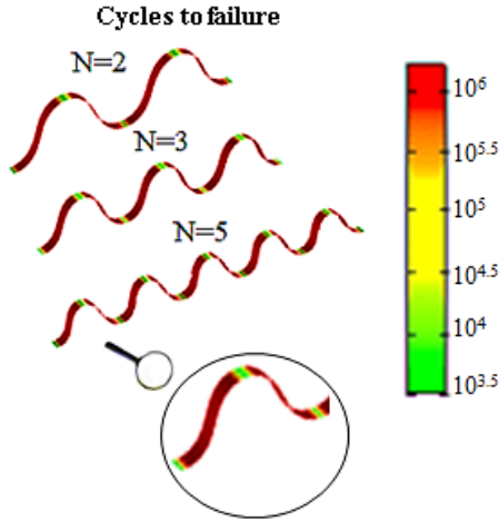
Fig. 7. Number of cycles to failure for the half wavelength dipole antenna on a PDMS substrate after release of 60% strain.
