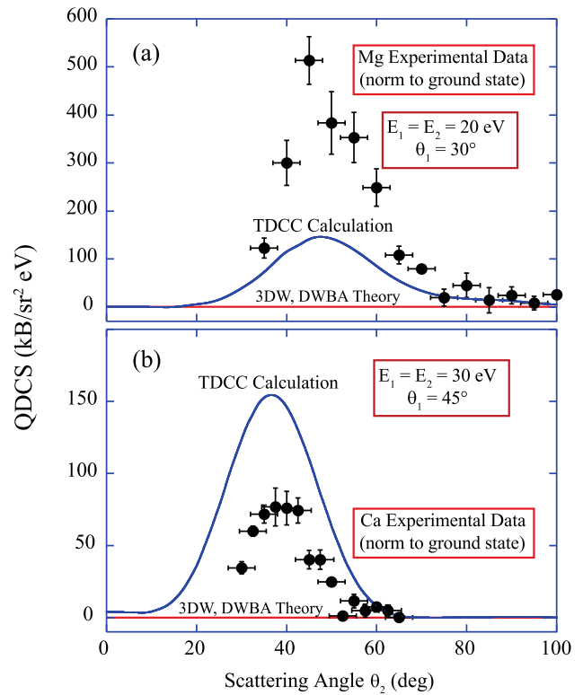
Figure 6. QDCS when \mathbf{k}_B is aligned orthogonal to the plane for (a) Mg and (b) Ca. Both 3DW and DWBA theories predict QDCS = 0 for all scattering angles. The TDCC calculation which includes un-natural parity states predicts a non-zero cross section, although the magnitudes do not agree with experiment. The data are normalized to results for ground state ionization.
