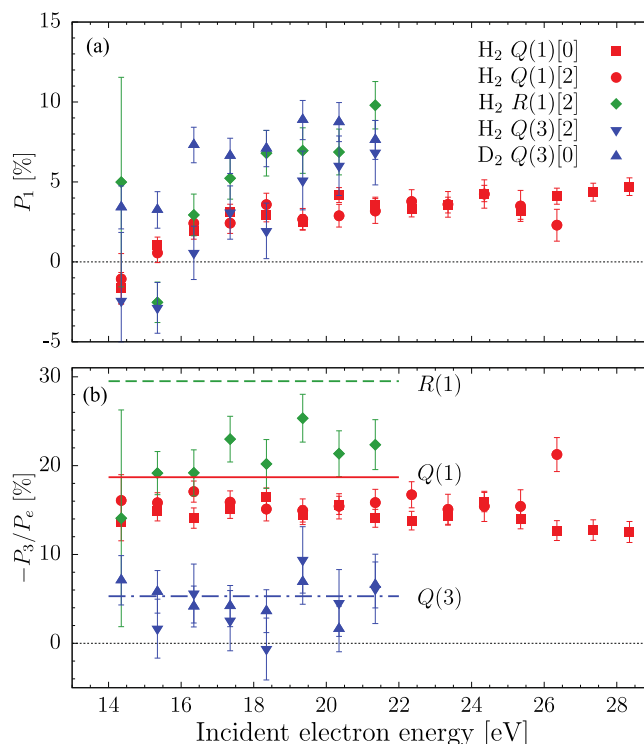
Figure 4. Linear (a) and circular (b) polarization fractions for the \text{H}_2 d^3\Pi_u \rightarrow a^3\Sigma_g^+ emission band. The circular-polarization data were normalized to the incident electron polarization and can be predicted approximately by using purely angular-momentum coupling [17], as shown by the straight lines. Reprinted with permission from [17], copyright 2013 by the American Physical Society.
