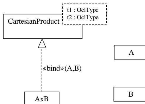
Figure 36 – Formation of a Cartesian Product AxB
