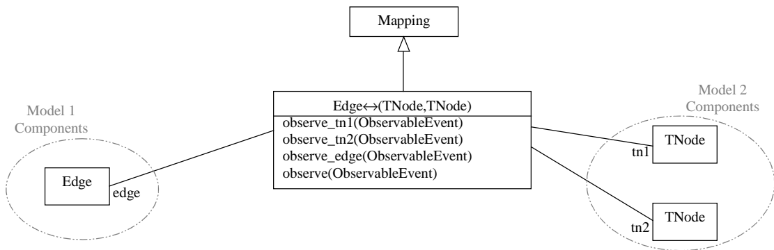
Figure 60 – Edge \leftrightarrow (TNode, TNode) Mapping Component
