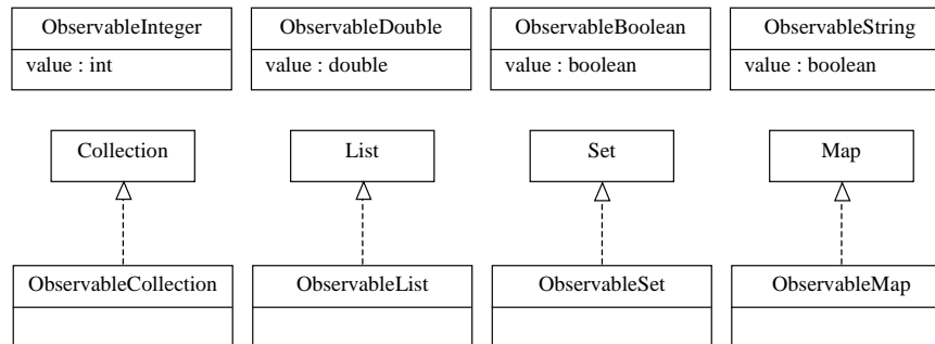
Figure 58 – Observable data and collection types
