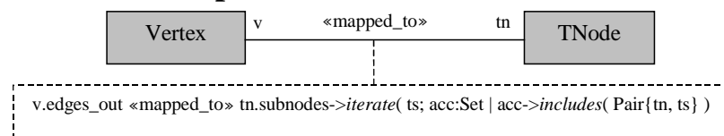
Figure 98 – Vertex↔TNode mapping specification
