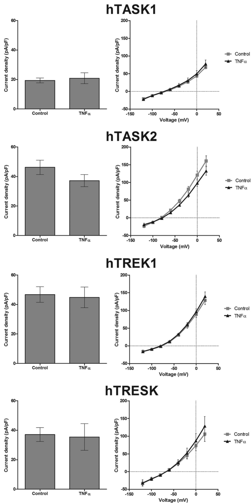
FIGURE 3. TNF \alpha does not affect hTASK1, hTREK1, hTASK2, and hTRESK1 currents. Graphs show various K 2 P channel current densities in untreated cells and cells treated for 2 h with TNF \alpha (10 ng/ml). The K 2 P current densities between -80 and -40 mV are on the left and the density of current-voltage plot on the right .
