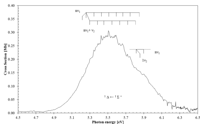
FIG. 2. VUV photoabsorption cross section in the 4.5–6.5 eV absorption band of COS.
