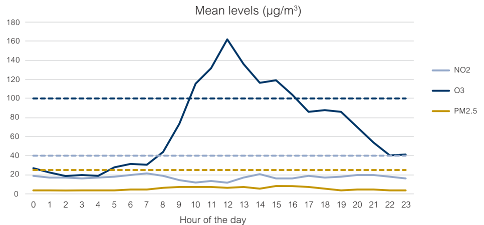
Figure 7: Hourly averages across both locations for NO 2 , O 3 , and PM 2.5 levels (July 5th 2018). Straight lines represent current legal annual average thresholds for each pollutant 4 (O 3 : 100µg/m 3 , NO 2 : 40µg/m 3 , PM 2.5 : 25µg/m 3 ).
