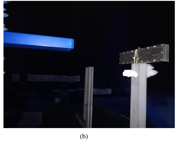
Fig.12. Photographs of the proposed filtering antenna. (a) Inner view; (b) 3-D view in the anechoic chamber
