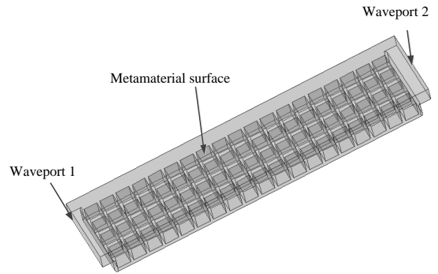
Fig. 4. Configuration of the filtering waveguide
