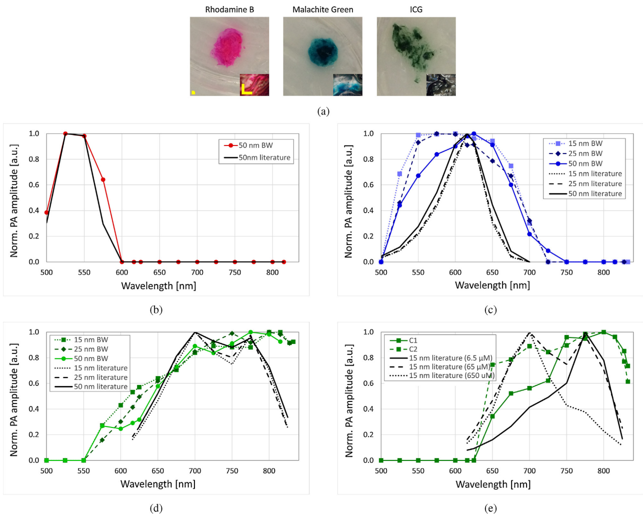
Fig. 4. (a) Photo of the three different samples, with microscopic image by reflection, scale bars 1 mm. Absorption spectrum adapted from the literature and inferred via photoacoustic measurements for different bandwidths (15 nm, 25 nm and 50 nm) of (b) Rhodamine B, (c) Malachite Green, (d) Indocyanine Green (ICG) (with literature corresponding to a concentration of 65 \mu\text{M} ) and (e) ICG for different concentrations with 15 nm bandwidth.
