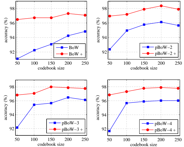
Figure 11. NAR fusion systems. Performance of the fusion systems compared to the baseline systems. Note that the fusion systems are denoted with the additional '+' symbol.
