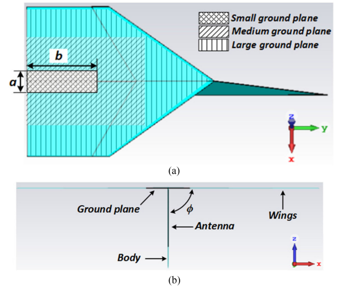
Fig. 5. Antenna optimized for a small ground plane. (a) Top view. (b) Back view.
