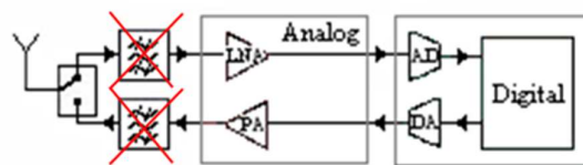
Figure 4 – Simplified UWB Transceiver
