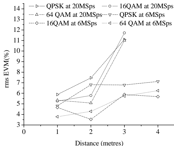
Fig. 8 – Uplink rms EVM measurements of emulated WiMAX schemes for different wireless distances. The lines between symbols are only an aid for viewing the results and do not represent predicted trends.
