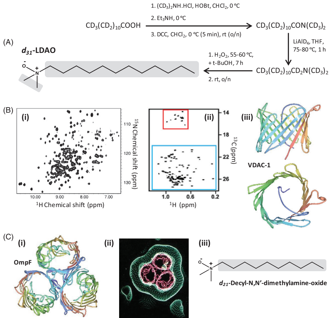
Figure 3. Synthesis of d_{31} -LDAO and its use in solubilizing the human voltage-dependent anion channel (VDAC-1) and use of tail-deuterated decyl- N,N' -dimethyl amine oxide in solubilizing Escherichia coli outer membrane protein OmpF. (A) Synthesis of d_{31} -LDAO from d_{23} -dodecanoic acid. The grey areas show the regions of deuteration. (B) (i) [ ^{15}\text{N} - ^1\text{H} ]-TROSY spectrum of [ \text{U}-^2\text{H} , ^{15}\text{N} ]VDAC-1 in d_{31} -LDAO micelles, (ii) [ ^{13}\text{C} - ^1\text{H} ]HMQC spectrum of [ \text{U}-^2\text{H} , ^{13}\text{C} , ^{15}\text{N} ; ^1\text{H}_8\text{-IL} ; ^1\text{H}_7\text{-V} ]VDAC-1 in d_{31} -LDAO micelles highlighting the spectral regions for Ile residues (red box, 11/11 assigned) and Leu plus Val residues (blue box, 8/12 Val and 17/28 Leu assigned), (iii) structure of human VDAC-1 shown as a side view (top) and from above (bottom) with the N-terminus in blue and C-terminus in red, which were drawn using PDB file 2K4T and PDB Protein Workshop 3.9 (Moreland et al., 2005). Pictures of the spectra were reproduced with permission from Hiller et al. (2008), which were originally published in Science (Hiller S, Garces RG, Malia TJ, Orekhov VY, Colombini M, Wagner G. 2008. Solution structure of the integral human membrane protein VDAC-1 in detergent micelles. Science 321:1206–1210, copyright by American Association for the Advancement of Science 2008). (C) (i) Crystal structure of the E. coli outer membrane protein OmpF in tetragonal crystal form as an above view with the N-terminus in blue and C-terminus in red, which was drawn using PDB file 1OPF and PDB Protein Workshop 3.9 (Moreland et al., 2005). (ii) Single-crystal neutron diffraction density map of OmpF in tail-deuterated decyl- N,N' -dimethyl amine oxide detergent contrast mapped parallel to the three-fold trimer axis where the porin trimer is represented by the \text{C}\alpha trace (pink) obtained from the X-ray crystal structure. This picture was reproduced with permission from Pebay-Peyroula et al. (1995), which was originally published in Structure (Pebay-Peyroula E, Garavito RM, Rosenbusch JP, Zulauf M, Timmins PA. 1995. Detergent structure in tetragonal crystals of OmpF porin. Structure 3:1051–1059, copyright by Elsevier Inc. 1995). (iii) Structure of the detergent d_{21} -decyl- N,N' -dimethyl amine oxide. The grey area shows the region of deuteration. This Figure is reproduced in colour in the online version of Molecular Membrane Biology .
