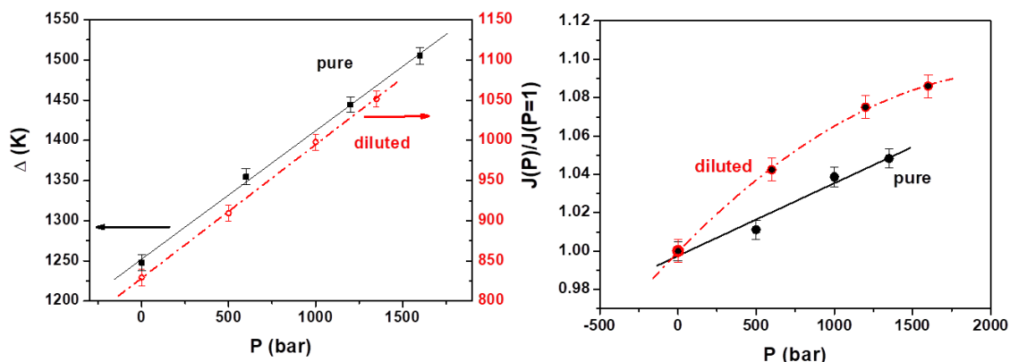
Figure 24. The pressure dependence of the average values of electronic gap (left) and interaction parameter J (right). Reprinted with permission from [186] Copyright 2011 by the American Physical Society
