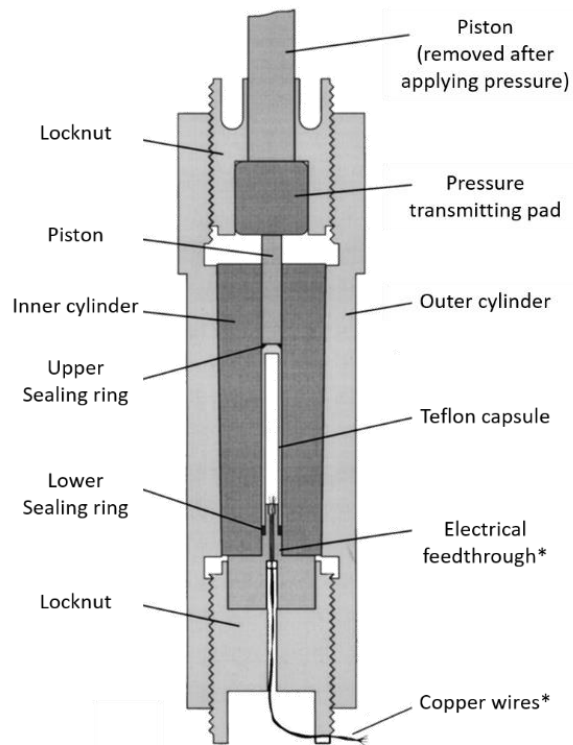
Figure 4. Cross-section of a typical clamp-type piston-cylinder pressure cell. Components marked * may only be used during pressure calibration. Reprinted from [108], with the permission of AIP Publishing
