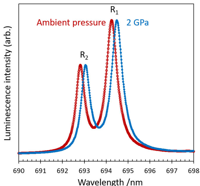
Figure 1. Illustration of the shift in position of the R1 fluorescence line of ruby on increasing pressure from ambient pressure to 2 GPa at room temperature
