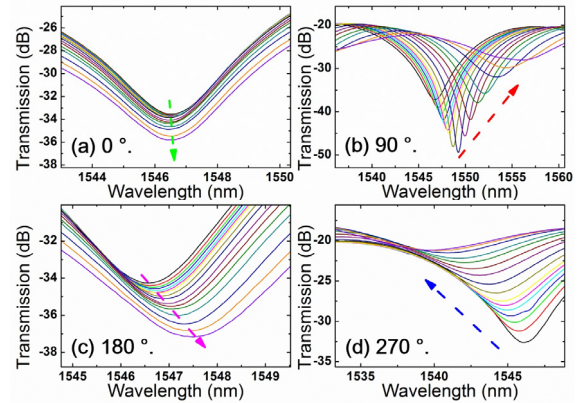
Fig. 5. Spectral evolution of dip B for different bending directions. (a) 0°. (b) 90°. (c) 180°. (d) 270°.
