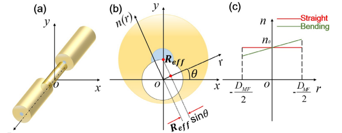
Fig. 3. (a) Unbent sensor in Cartesian coordinate system. (b) Fiber cross sectional geometry of the sensor bent in r axis. (c) Fiber cross sectional RI distribution in r axis.
