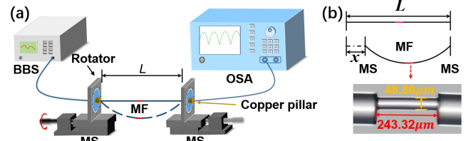
Fig. 2. (a) Experimental setup of the MAMZI-based vector bending sensing system. (b) Sketch for curvature calculation.
