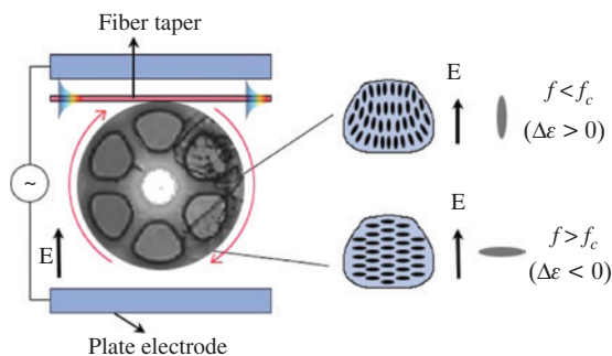
Figure 5: Cross-section of the grapefruit-MOF-based microresonator sandwiched between two electrodes and effect of an electric field on a DFLC at different frequencies.
