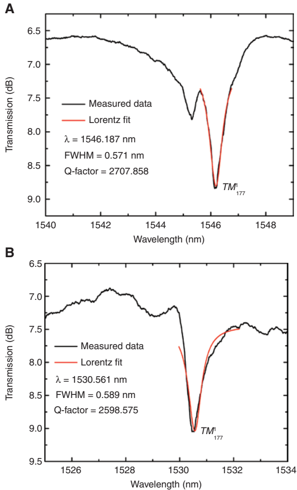
Figure 4: Lorentzian fitting of the WGM transmission spectra for TM_{177}^1 modes with estimated Q-factors for the two grapefruit MOF microresonators, respectively, infiltrated with (A) DFLC-1 and (B) DFLC-2 in the absence of electric field at room temperature.
