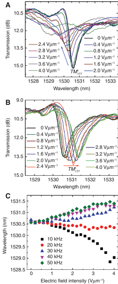
Figure 7: Transmission spectra of the grapefruit-MOF-based microresonator filled with DFLC-2 under the applied electric field at (A) 10 kHz and (B) 50 kHz, respectively. Arrows in these figures indicate the spectral shift direction with the increment of the applied electric field intensity. (C) WGM resonance wavelength shift as functions of applied electric field for different AC signal frequencies.
