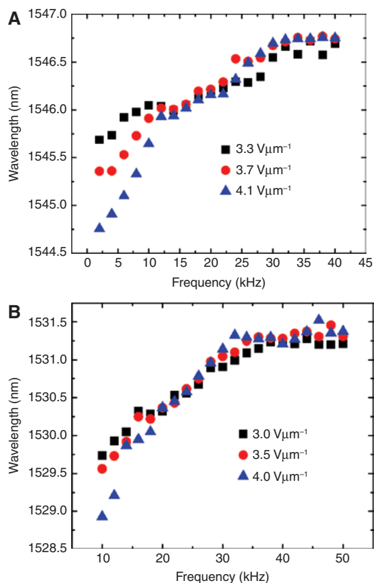
Figure 8: WGM resonance wavelength as functions of applied electric field frequency under different electric field intensities for grapefruit-MOF-based microresonators filled with (A) DFCL-1 and (B) DFCL-2, respectively.
