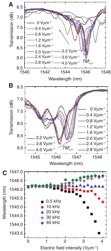
Figure 6: Transmission spectra of the grapefruit-MOF-based microresonator filled with DFLC-1 under the applied electric field at (A) 0.5 kHz and (B) 40 kHz, respectively. Arrows in these figures indicate the spectral shift direction with the increment of the applied electric field intensity. (C) WGM resonance wavelength shift as functions of applied electric field for different AC signal frequencies.
