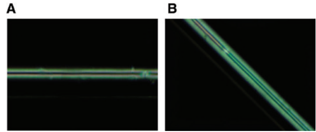
Figure 2: Polarized micrographs of silica capillaries (inner diameter, 30 \mu\text{m} ) infiltrated with DFLCs. Capillaries angled at 0° (A) and 45° (B) with respect to the polarizer axis.
