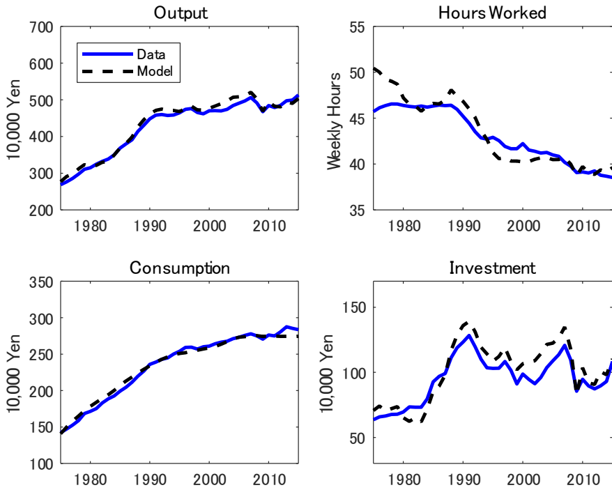
Figure 6: Benchmark Simulation
