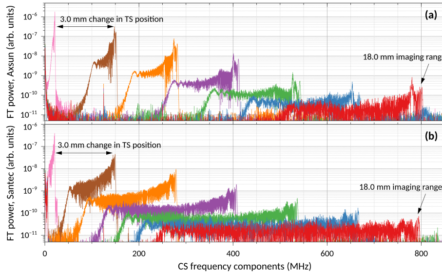
Fig. 4. Comparison of the frequency spectra of the channeled spectra obtained at 7 different OPDs (with a spacing of 3.0 mm between them) for the Axsun source (top plot, (a)) and for the Santec source (bottom plot, (b)). All data sets sampled with the DSO, set at 5 GS/s sampling rate.
