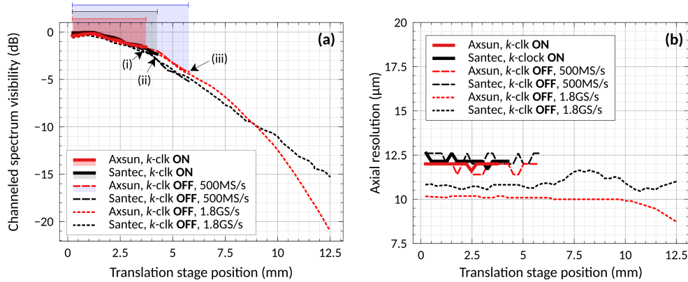
Fig. 2. (a) Channelled spectrum (CS) visibility versus TS position (obtained with the CMS method), measured for the case with the k -clock enabled (continuous lines) and for two other data sets with the k -clock disabled, acquired with a digital sampling rate of 500 MS/s (large dashes) and 1.8 GS/s (short dashes); red trace: Axsun source; black trace: Santec source. The shaded regions denote the axial range attainable with the Axsun using the k -clock (red), the Santec using the k -clock (grey), and either source without the k -clock and a 500 MS/s sampling rate (light blue). (b) Axial resolution estimated from the A-scan peak FWHM for the same cases described in (a).
