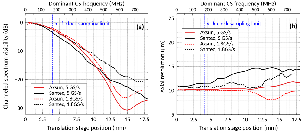
Fig. 3. (a) Channelled spectrum (CS) visibility versus TS position (obtained with the CMS method), measured for the data sets acquired with either the DSO (continuous lines) and the ATS sampling at 1.8 GS/s (dashed lines); red traces correspond to the Axsun source, whereas black traces correspond to the Santec source. (b) Axial resolution estimated from the A-scan peak FWHM for the same cases described in (a). Top axis shows the dominant (peak) frequency in the channelled spectrum for each TS position, obtained via a FFT-based analysis. Blue vertical line in either plot shows the axial imaging limit imposed by the k -clock (350 MHz, corresponding to a channelled spectrum frequency of 175 MHz).
