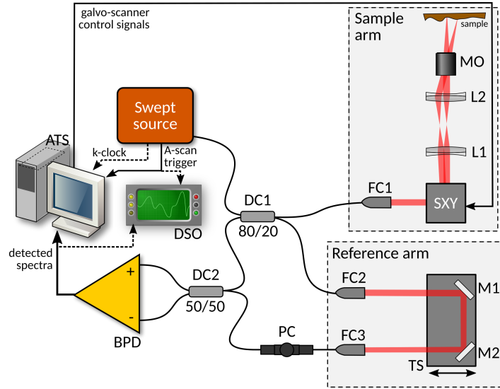
Fig. 1. Swept-source OCT system used to demonstrate the long axial range CMS interferometry procedure. DC1-2: fiber-based directional couplers; FC1-3: fiber collimators; SXY: pair of galvo-scanners (Cambridge Technologies, model 6110); L1-2: achromatic lenses forming a telecentric configuration; MO: microscope objective; M1-2: flat protected silver mirrors; BPD: balanced photo-detector; PC: fiber-based inline polarization controller; TS: translation stage; ATS: AlazarTech ATS9360 digitizer board (inside computer); DSO: digital storage oscilloscope.
