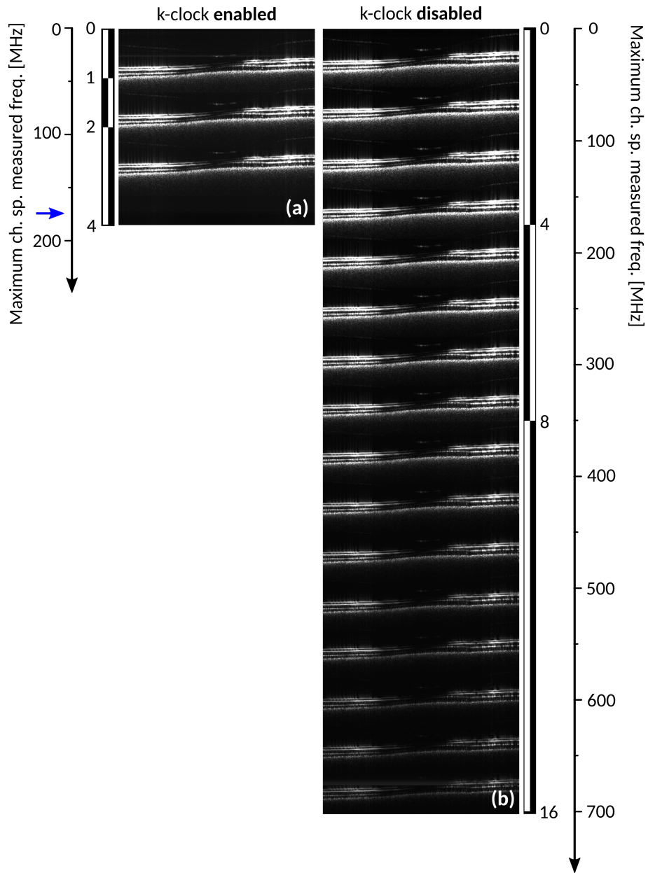
Fig. 5. Composite image generated from multiple B-scans, each taken at a different OPD setting with the Axsun source (separated by 1 mm in between B-scans). (a) B-scans acquired while using the source k -clock; (b) B-scans acquired by sampling the data at 1.8 GS/s using the ATS clock instead of the swept source k -clock. Scale bar units: mm. Transversal span is \sim 1 mm. Blue arrow: maximum frequency attainable with the k -clock of the Axsun source (175 MHz, corresponding to a sampling rate of 350 MHz).
