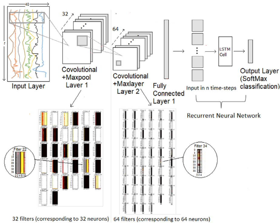
Fig. 4. CNN-LSTM Model Architecture, we train 4 models separately, these are (a) On-Body, (b) Env , (c) for Location (d) and then we fused model using all the data input and feed it into the Deep Layers.
