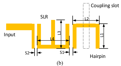
FIGURE 5. Configuration of the proposed low frequency-ratio DBDP filtering antenna (Antenna-I): (a) exploded view; (b) feeding resonators of each polarization. Lp = 17.8 mm, Lg = 50 mm, Ls1 = 11.8 mm, Ls2 = 10.3 mm, Ws = 0.9 mm, L1 = 5.8 mm, L2 = 4 mm, L3 = 7 mm, L4 = 6.5 mm, S1 = 1.2 mm, S2 = 0.3 mm.
