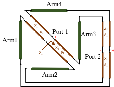
Fig. 20. Equivalent circuit of highly integrated DPSD antenna.
