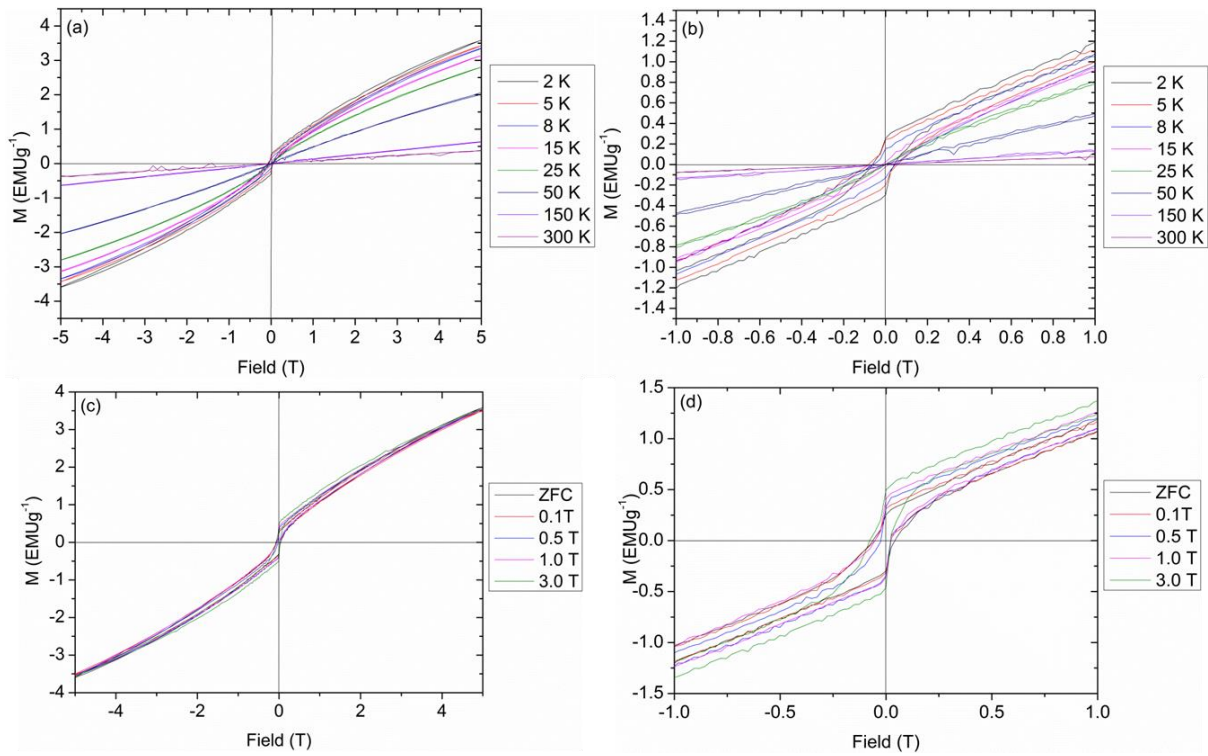
Figure 8: (a) Zero field cooled hysteresis data collected at temperatures between 2 K and 300 K showing the loss of hysteric behaviour above ~50 K, (b) zoomed in region of the data shown in (a), field cooled hysteresis data collected at 2 K as a function of cooling field strength showing the increase in remnant magnetisation with increasing cooling field strength and (d) zoomed in region of the data shown in (c) (Colour online).
