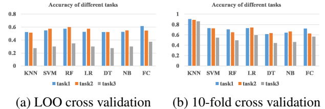
Fig. 4. The accuracies of different tasks. Among them, task1 (high/low valence), task2 (high/low arousal), task3 (low arousal low valence/high arousal low valence/low arousal high valence/high arousal high valence)
