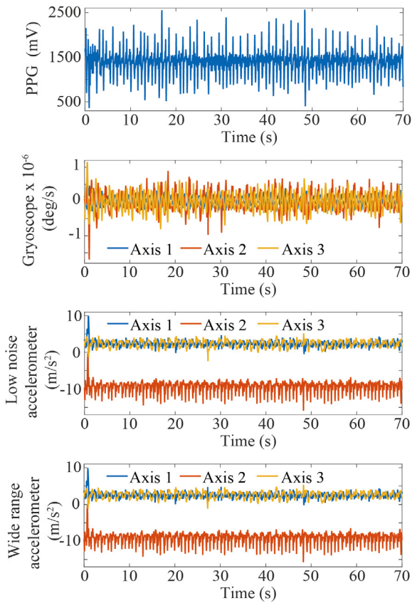
Fig. 3. PPG, gyroscope and accelerometers during walking.
