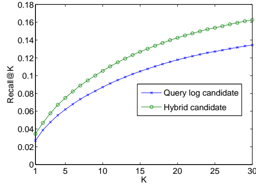
Fig. 9. Comparison of two candidate options, namely, query log candidate and hybrid candidate for addition operation.
