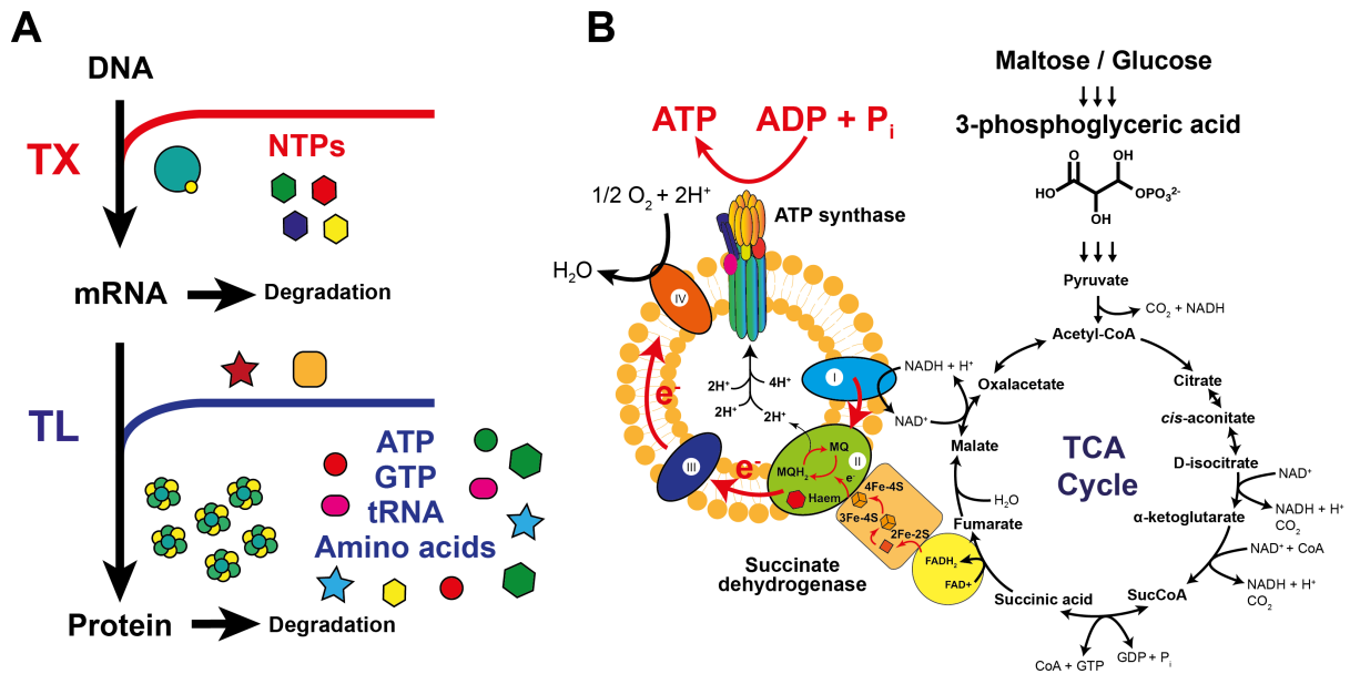
Figure 1. Summary of cell-free transcription-translation. A, Transcription (TX) and translation (TL) process and requirements of nucleotide triphosphates (NTPs) and substrates (ATP, GTP, tRNA and amino acids). B, Energy regeneration cycle for central metabolism. ATP is synthesised through the formation of inverted vesicles, which spontaneously form during cell-disruption [37] . Abbreviations: MQ, menaquinone; MQH 2 , reduced menaquinone.
