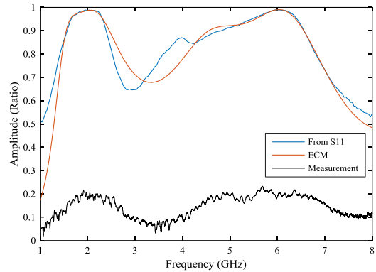
Fig. 4. Amplitude of S_{21} from the ECM, from S_{11} , and from measurement.
