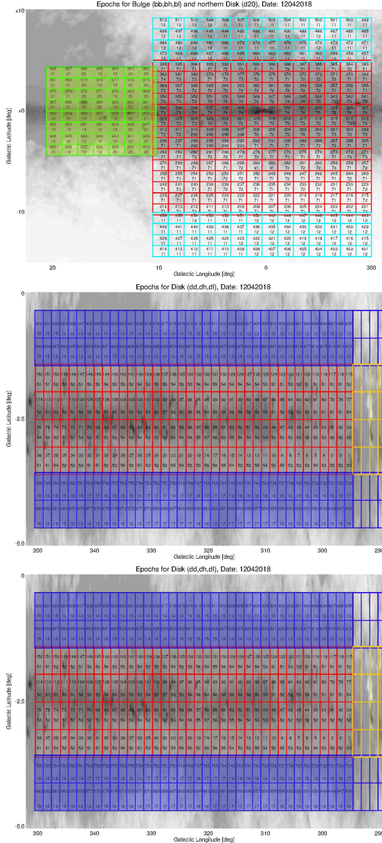
Figure 1. The VVVX Survey area. The red squares show the VVV Survey tiles, the green – the Northern disk extension, the cyan – the bulge area extension, the blue – the extensions of both sides of the South VVV disk, and the yellow – new VVVX outer disk fields. The searched areas are filled with green and dark blue colors. The numbers in each tile are its identification number (top) and the number of K_S epochs by April 12, 2018.
