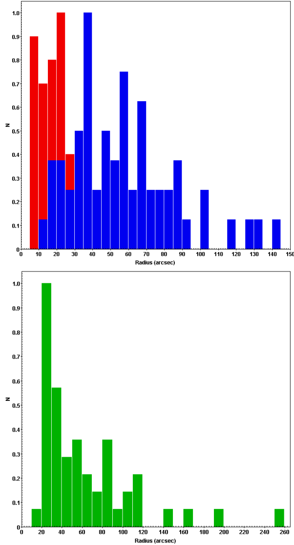
Figure 6. Distribution of the detected objects with measured cluster radius (given in arcsec). The red color stands for young/embedded clusters, while the blue one is for open ones. The second panel shows known clusters in the VVVX area.
