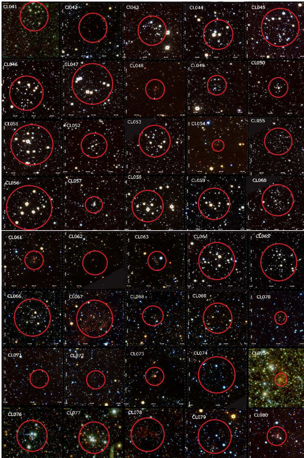
Figure C1 – continued VVVX JHK_S composite color images of the open cluster candidates.
