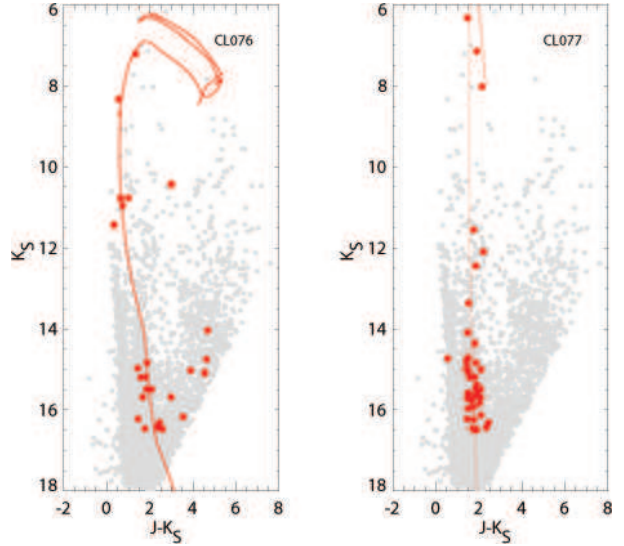
Figure 3. The VVVX CL076 and CL077 K_S vs (J - K_S) diagram, with most probable cluster members (red large circles) overplotted (see text). The solid red lines are best fit solar isochrones of 32 and 10 Myr, respectively, taken for Padova database.
