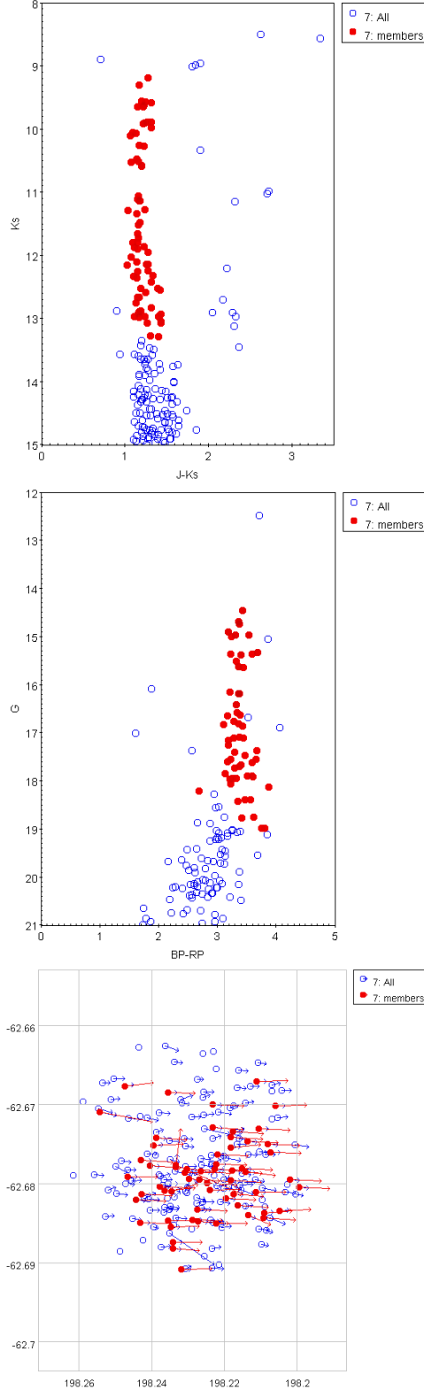
Figure 4. The VVV and Gaia DR2 color magnitude and proper motion diagrams with sky vectors overlotted for known open cluster Danks 2. Blue open circles are all stars in the selected area, the red solid ones stand for most probable cluster members. The proper motion vectors are scaled by factor of 2 for visibility.
