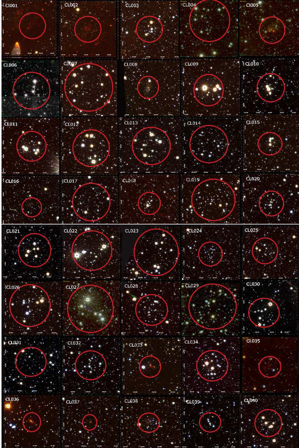
Figure C1. VVVX JHK_S composite color images of the open cluster candidates. The field of view is 2.5 \times 2.5 arcmin, north is up, east to the left.
