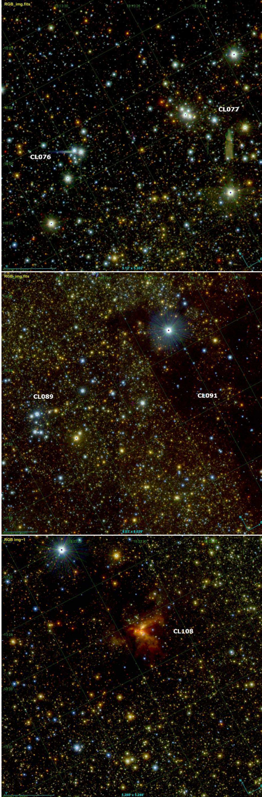
Figure 2. VVVX JHK_S composite color images of some open cluster candidates. The field of view is 5 \times 5 arcmin.
