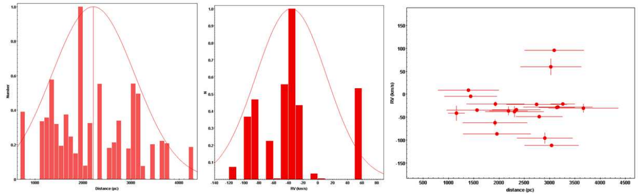
Figure 8. The histograms of distance and radial velocity distribution. The right panel shows RV vs Distance relation. The solid lines are Gaussian distribution.
