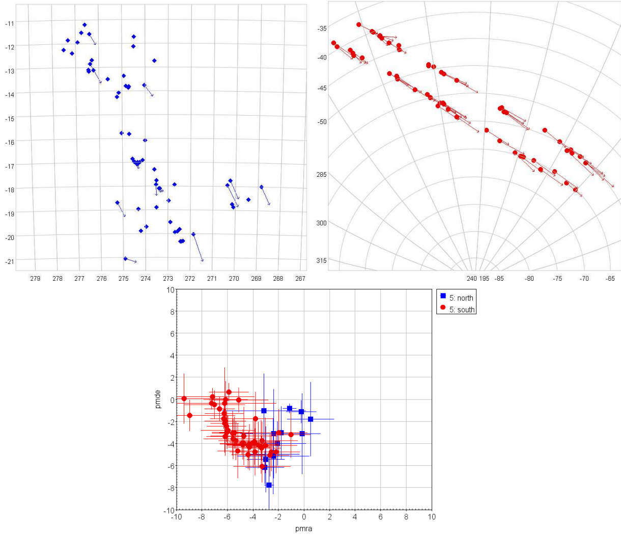
Figure 7. The diagram of mean proper motions of the cluster candidates. The blue squares are for the candidates projected in North disk VVX area, while red circles stand for the Southern part. The proper motion vectors are scaled by factor of 2 for visibility.
