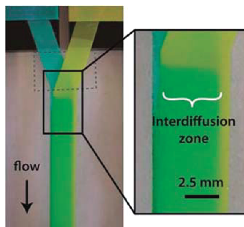
Figure 7. Demonstration of mixing in a flat Y-geometry paper mixer. Reproduced from ref 148 [ http://dx.doi.org/10.1039/c004821f ] by permission of The Royal Society of Chemistry.
