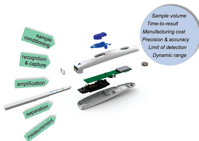
Figure 5. In POC microanalytical systems, unit operations (left-hand side) and overall system specifications (right-hand side) interact such that decisions on one element affect all others. This pregnancy-test device includes optical measurement with digital readout of the LFA-based single-use stick located at left. Device image courtesy of Unipath, Ltd.
