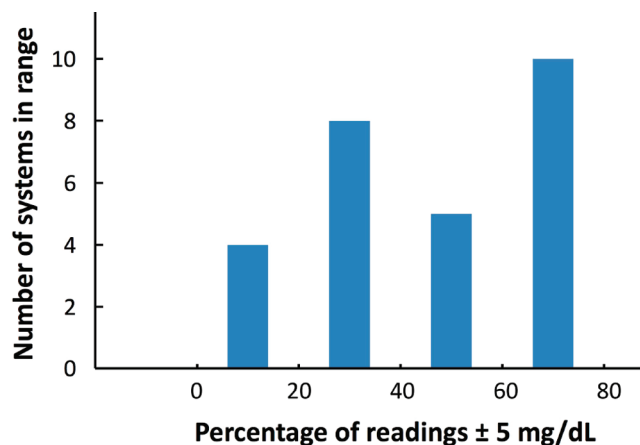
Figure 3. Performance of commercial self-test glucose measurement systems, determined under controlled laboratory conditions. Compiled from data tabulated in ref 70.
