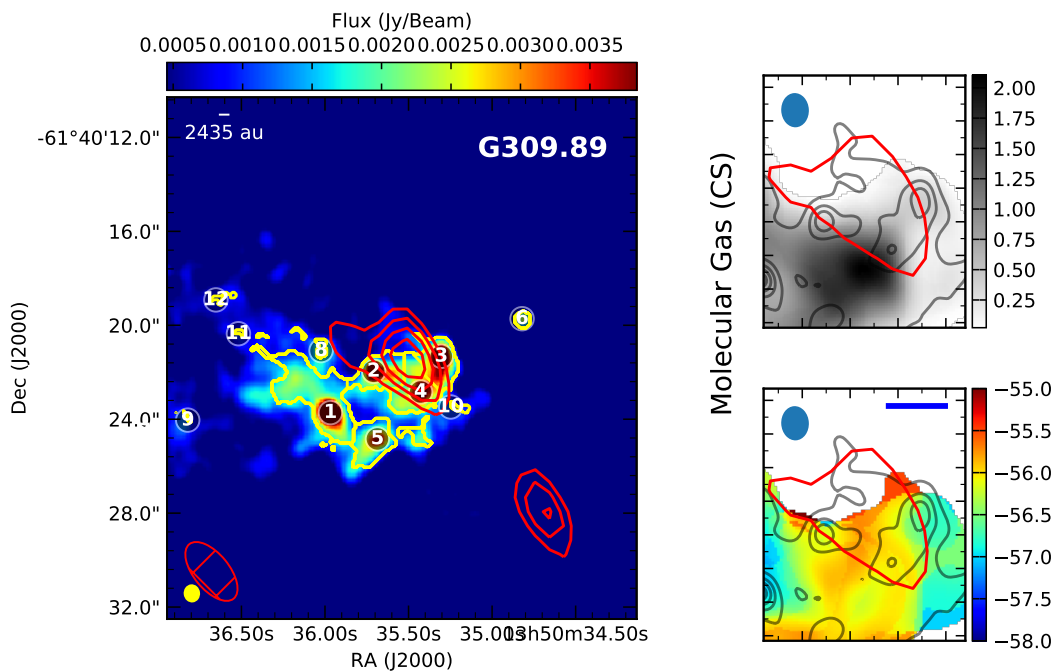
Fig. 8: Continuum and CS emission from G309.89. The left panel shows the 256 GHz continuum in colour scale with 5 GHz emission in red contours. The yellow contours show the outlines of the FellWalker identified cores. The two right panels show the moment 0 and moment 1 (top and bottom, respectively) maps of the CS emission focussed on the brightest clump, where the HII region is expected to be (although no H 2 9 \alpha was detected, the 5 GHz continuum shows its location).
