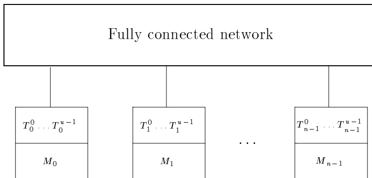
Figure 4: The multithreaded module parallel computer
