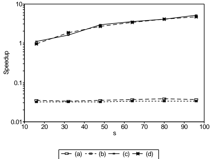
Figure 9: Speedup versus s for simulator SIM1 ( s \times s is the size of matrices A , B and C ; (a) and (b) — matrices A , B , C in the shared memory, h is a polynomial of degree 1 and 3, respectively; (c) and (d) — only matrix C in the shared memory, h is a polynomial of degree 1 and 3, respectively)
