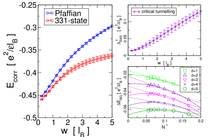
FIG. 4: (color online) Energies in the thermodynamic limit for the (3,3,1) and Pfaffian states at \nu = 1/2 (left). Data shown is for the infinite square well as a function of the well width w . The correlation energies are shown with respect to the single component background. In the absence of tunneling, the (3,3,1)-state has lower energy at all w . The critical tunneling strength required to favor the Pfaffian state (top right) and a few typical differences in the extrapolation of the background energies for different values of the well width (bottom right).
