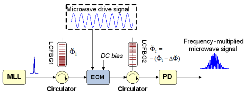
Figure 9. Schematic an unbalanced TPS system for microwave arbitrary waveform generation based on frequency multiplication. MLL: mode-locked laser, LCFBG: linearly chirped fiber Bragg grating, EOM: electro-optic modulator, PD: photodetector.
