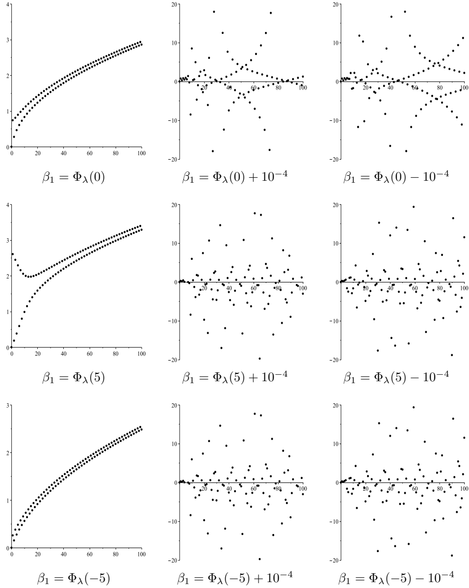
Figure 5.3: Plots of the points (n, \beta_n) where \beta_n satisfies (5.2) with initial conditions \beta_0 = 0 and \beta_1 = \Phi_\lambda(t) + \varepsilon , with \Phi_\lambda(t) given by (2.2), and \varepsilon = 0, \pm 10^{-4} , for t = 0, \pm 5 and \lambda = \frac{1}{2} .
