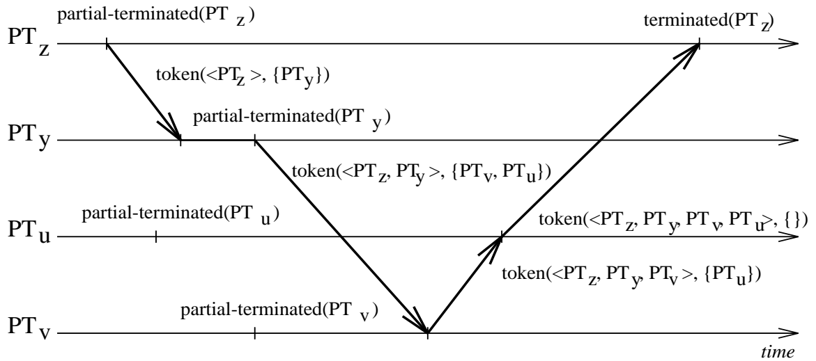
Figure 24: Token Algorithm.
