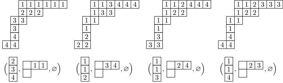
FIGURE 2. The bijection in Proposition 3.6 between border-strip tableaux of shape (8, 5, 3, 2, 2)/(2, 2, 1, 1, 1) and type (6, 3, 3, 3) and 3-quotient border-strip tableaux of the same shape and type (2, 1, 1, 1) . The shapes of the border-strip tableaux forming each 3-quotient border-strip tableau are given by the 3-quotient of (8, 5, 3, 2, 2)/(2, 2, 1, 1, 1) , namely ((1, 1, 1), (3, 1)/(1, 1), \emptyset) . To make clear the skew-shape, the tableaux of shape (3, 1)/(1, 1) are drawn as (3, 1) -tableaux with two empty boxes.
