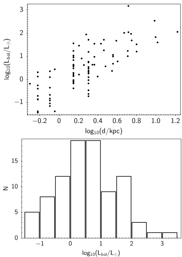
Figure 11. (Upper panel). Estimated bolometric luminosity vs distance for likely YSOs with 2–22 \mu\text{m} detections. Luminosities are based mainly on the 2010 epoch of 3–22 \mu\text{m} data from the WISE All-Sky catalogue. (Lower panel). Histogram of estimated bolometric luminosity.
