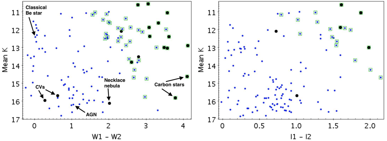
Figure 7. Colour magnitude diagrams for non-YSOs. ( Left ): Mean UGPS K vs WISE W1-W2 . ( Right ): Mean UGPS K vs Spitzer /IRAC I1-I2 . The IRAC I1 and I2 data are a little deeper than WISE W1 and W2 but they do not cover the full area of the UGPS catalogue. Known variables are marked in black and variables in our dusty AGB star selection region in figure 8 are enclosed in green squares. Dusty AGB stars mostly found at the upper right. The nature of the small group of bright blue variable stars in the left panel is unclear, see text. The larger group of faint variables includes both faint red stars (some of which will be relatively isolated YSOs) and faint blue variables such as CVs, EBs and AGN, seen in greater numbers in the upper left panel of figure 5.
