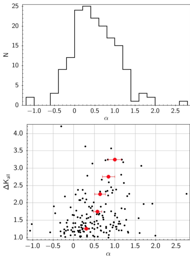
Figure 9. (Upper panel): histogram of the distribution of 2-22 \mu\text{m} spectral index, \alpha . (Lower panel): Amplitude \Delta K_{all} vs \alpha . YSOs with larger amplitudes show a subtle tendency to have redder spectral indices, as illustrated by the large red points corresponding to the median of \alpha in amplitude bins of width 0.5 mag, up to \Delta K_{all}=3.25 . Error bars represent the standard error, \sigma/\sqrt{N} .
