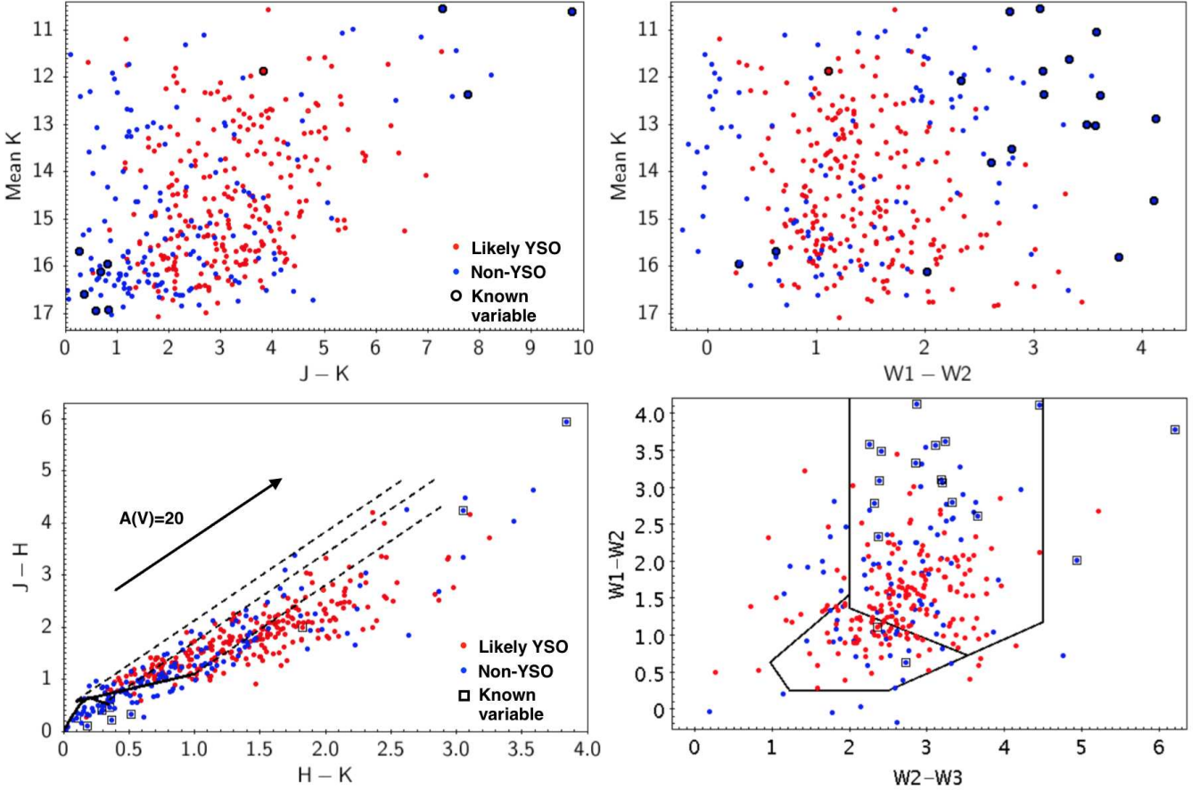
Figure 5. CMDs and two colour diagram for likely YSOs (red points) and non-YSOs (blue points). Known variables are circled in black circles in the upper panels and black squares in the lower panels. ( upper left ): mean UGPS K vs. J - K . ( upper right ): mean UGPS K vs. W1 - W2 . ( lower left ): near infrared two colour diagram, with dashed lines illustrating the reddening paths from the classical T Tauri locus (solid line) and the main sequence (curve). Reddened main sequence stars should lie between the left and central dashed lines, whereas classical T Tauri stars may lie between the left and right dashed lines. Protostars and other stars with large amounts of circumstellar matter may lie to the right of all the dashed lines. ( lower right ): W1 - W2 vs. W2 - W3 , with solid lines enclosing the typical locations of class I YSOs (upper part) and class II YSOs (lower part), see Koenig & Leisawitz (2014) . The locations of the likely YSOs in the lower panels support their position-based classification. Known variables are mostly dusty AGB stars (sources redder than most YSOs, often undetected in J ) or CVs (faint blue sources, often undetected in W1 and W2 ).
