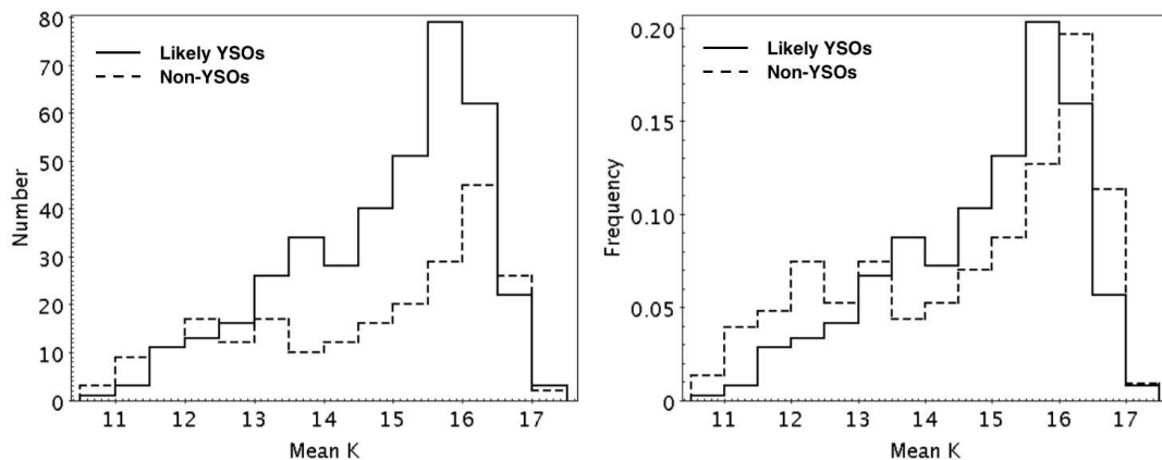
Figure 6. Mean UGPS K magnitude distributions for likely YSOs and non YSOs. ( left ) Absolute numbers ( right ) Normalised distributions, each with unit area.
