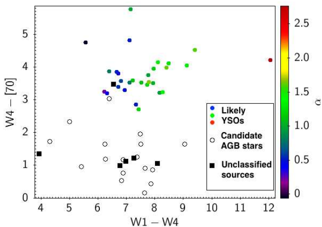
Figure 10. Separation of variable YSOs and dusty Mira variables in the W4-[70] colour. The W4-[70] vs. W1-W4 two colour diagram shows a fairly clean separation of YSOs (filled circles) and AGB stars (open circles), supporting our position-based YSO selection method and our mid-infrared selection method for dusty AGB stars. Unclassified sources (filled black squares) mostly lie amongst the AGB stars. The YSOs are colour-coded by spectral index, which is closely correlated with the W1-W4 colour.
