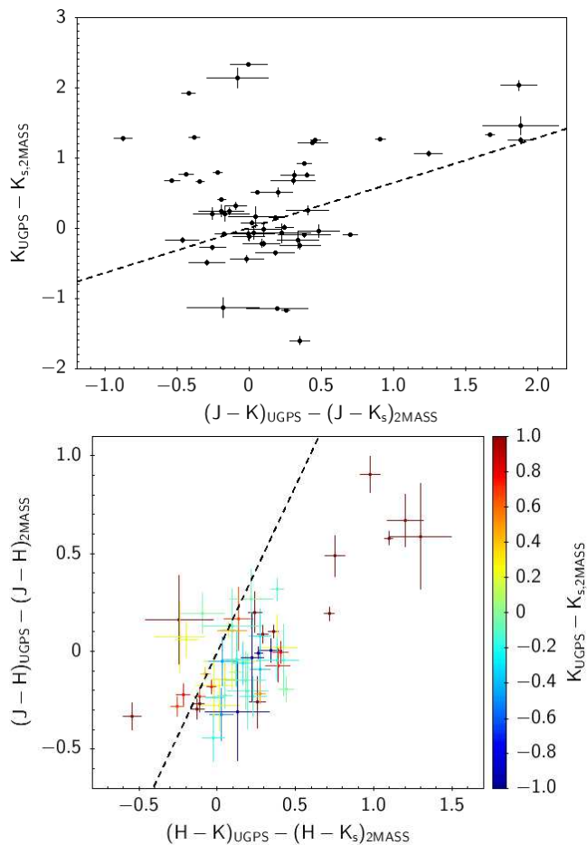
Figure 13. Colour variability. ( Upper panel ): plot of change in flux vs. change in colour between UGPS and 2MASS. The reddening track is overlaid as a dashed line. Most sources are fainter in UGPS than 2MASS due to greater survey sensitivity. A few sources with large flux changes lie close to the reddening line but most do not. ( Lower panel ): two colour diagram of colour changes between UGPS and 2MASS, with extinction track overlaid and the change in flux colour coded. Sources with a large 2MASS:UGPS reddening increase show larger changes in H - K than would be expected from extinction alone. Some sources at the lower left also became fainter while becoming bluer on both axes.
