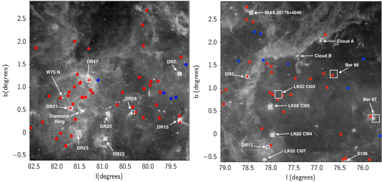
Figure 14. The Cygnus X spatial group. The greyscale background is the 8.3 \mu\text{m} image data from the MSX satellite. The two panels include almost all of the group. Red circles are likely YSOs and blue circles are other sources. Infrared-bright SFRs are labelled, along with selected well known HII regions and pre-MS clusters from Downes & Rinehart (1966) and Le Duigou & Knödlseher (2002) that are located close to variable sources. (Clusters and radio sources are marked with squares, with larger squares for the larger clusters). In the left panel we see that most of the likely YSOs are located either in the active region of star formation around W75 N, DR21, DR17, DR23 and the Diamond Ring or within the Cyg OB2 association centred near l = 80^\circ . In the right panel there is some concentration of likely YSOs near the LK02 Cl03 cluster and near the upper left portion of the large IR-bright ring that extends from Clouds A and B through DR5, DR13 and down to S106 (see Schneider et al. 2007 ). However, some likely YSOs are associated with smaller SFRs that are not apparent on this scale.
