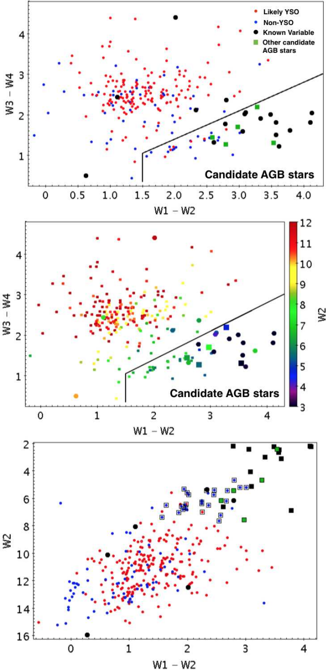
Figure 8. Selection of candidate AGB stars. ( Top ): WISE two colour diagram with likely YSOs in red, non-YSOs in blue, known variables as large black points and other candidate AGB stars from the literature as large green squares. The known variables are mainly dusty AGB stars located at lower right, save for a CV at lower left, a PN central star at top and a candidate eruptive YSO at centre left. The dividing line encompasses most of the known AGB stars while including only five sources projected against SFRs. ( Middle ): as upper panel but with W2 mag colour coded to illustrate how the simple colour selection picks out the brightest mid-infrared stars. ( Bottom ): W2 vs. W1-W2 colour magnitude diagram with the same colour coding as the upper panel. The 42 sources in the AGB selection region are enclosed in squares.
