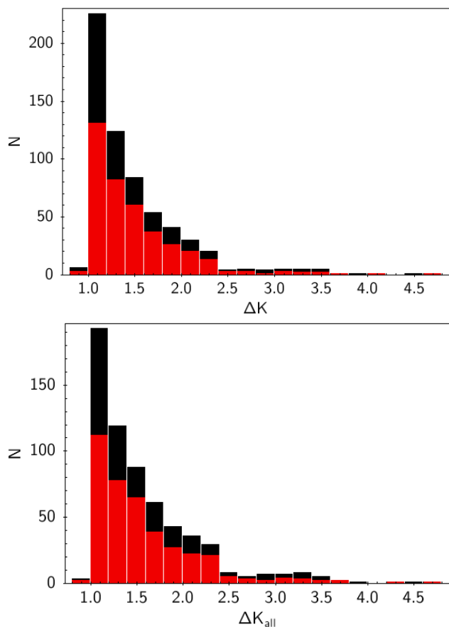
Figure 3. Distribution of amplitudes for the 618 variable stars in the catalogue. ( upper panel ): two-epoch amplitude \Delta K from UGPS. ( lower panel ): amplitude \Delta K_{all} , which includes a 3rd epoch of photometry in K_s from 2MASS, where available. The subset classified as likely YSOs is shown in red. A few sources have \Delta K=0.98-1.00 due to small calibration adjustments between the FITS catalogue photometry and DR10, see Appendix B.
