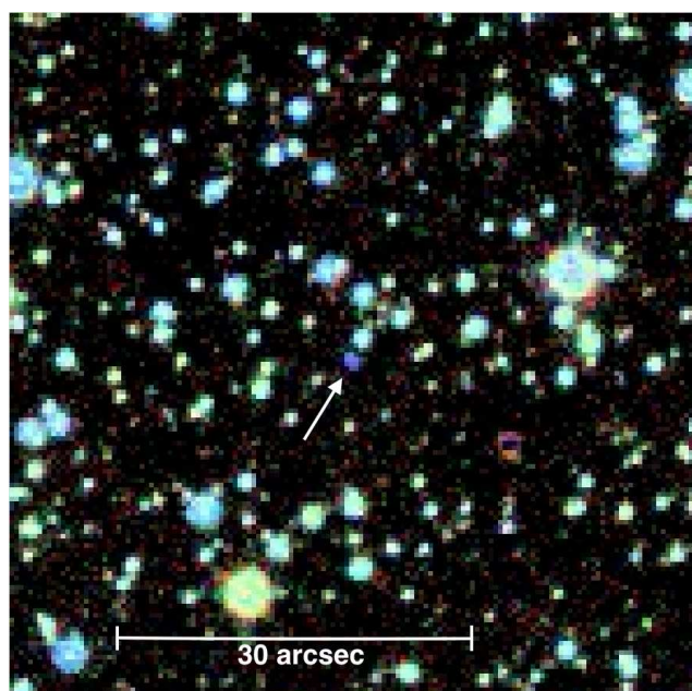
Figure 16. UGPS near infrared three colour image of source 363 (July 2010 data, with red, green and blue represent K , H and J , respectively). The source is indicated with an arrow and the image has conventional equatorial orientation. The deep blue colour of the object reflects the extreme measurement J - H = -0.6 .
