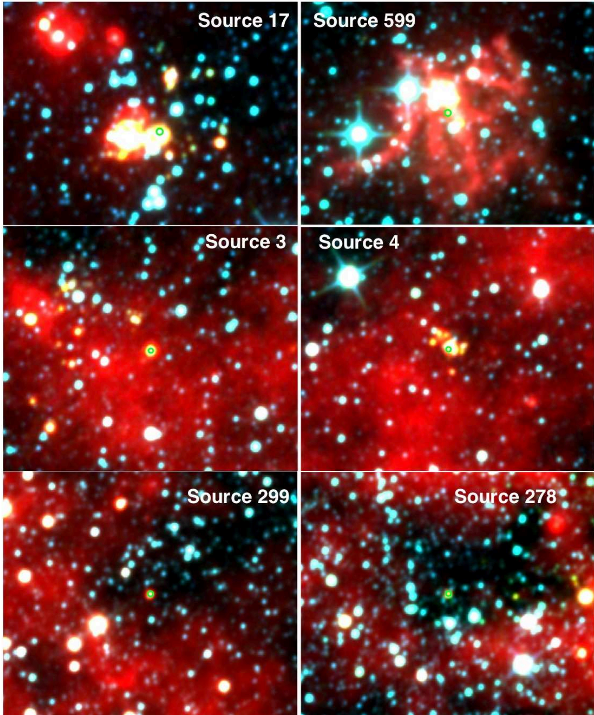
Figure 4. Examples of YSO/non-YSO classification using WISE three colour images: W1 ( 3.3 \mu\text{m} , blue), W2 ( 4.6 \mu\text{m} , green), W3 ( 12 \mu\text{m} , red). Normal stars usually appear blue whereas YSOs often appear red, yellow or green. Each image is 10' across with north at the top and east at left. The variable stars are marked with a green circle at the centre of each panel, though not all are clearly seen in WISE. The variables in the top and middle panels are classified as likely YSOs but those in the lower panels are not. Source 17 is in the clearly apparent pre-MS cluster [FSR2007] 0671 (Froeblich et al. 2007) so the WISE image was not required. Source 599 is in a previously uncatalogued SFR and likely HII region associated with IRAS 21401+5228, see section 4.3. Source 3 is at the edge of a small uncatalogued group or cluster of pre-MS stars centred on IRAS 03262+5536. Source 4 is in a marginally resolved uncatalogued group of YSOs. Sources 299 and 278 are in inner Galaxy mid-plane fields where YSO identification is more difficult. The field around source 299 contains several bright stars that have red edges but most of these are probably distant AGB stars (see text). The source 278 field contains several rather faint green sources in the dark area at right of centre. This is likely an IRDC but it is unclear whether the green stars are YSOs or background stars.
