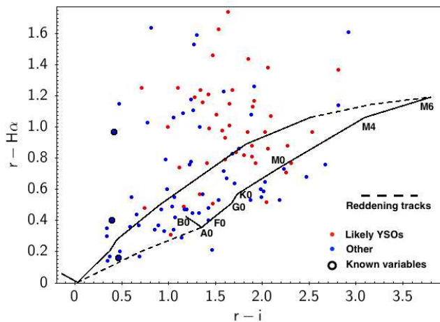
Figure 12. IPHAS r-H\alpha vs. r-i two colour diagram. Solid lines show the main sequence tracks from B0 to M6, with zero reddening (left track) and E(B-V)=2 (right track). Red points are likely YSOs, most of which show clear evidence for H\alpha emission, based on location above both tracks. Blue points are other variables, almost half of which are also clearly H\alpha emitters. The three known variables plotted are enclosed large black circles: the central star of the Necklace nebula, dwarf nova EG Lac and Nova Cyg 2008, in descending order of r-H\alpha . The lower and upper dotted lines are the reddening tracks for A0V and M6V stars respectively.
