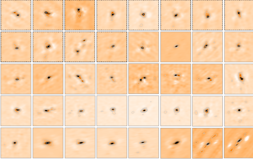
Fig. 1. Line-free continuum observations at 870\ \mu\text{m} of 40 of the targeted sources with ALMA ACA at 3\text{--}5'' angular resolution.
